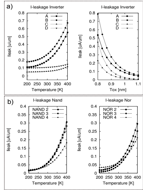
Fig. 5. TAMTAMS output (LEVEL2): a) leakage current of an inverter according to four of device currents models adopted: A) I_{gate} -Mastar and I_{off} -Mastar (no I_{btt} ); B) = I_{gate} -Mastar, I_{off} -Mastar, I_{btt} -Roy ([15]); C) I_{gate} -Lee, I_{off} -Fjedly; D) I_{gate} -Lee, I_{off} -Fjedly, I_{btt} -Roy. b) leakage current of a NAND gate (left) and a NOR gate (right) according to original MASTAR models of device currents. Different curves represent different number of inputs for each gate. In both cases: parametric analysis. Examples: left, current as a function of temperature; right, current as a function of a variation on gate oxide thickness.
