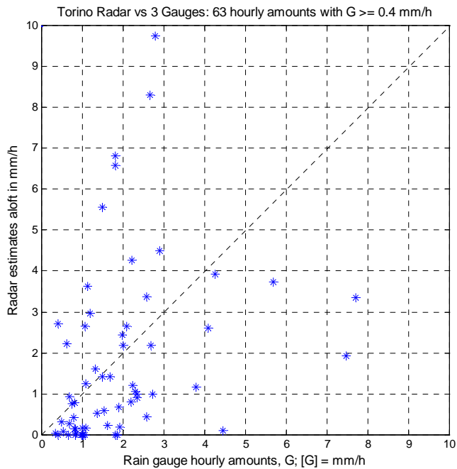
Fig. 17. Same as Fig. 7, but for the Torino radar (63 hours with G \geq 0.4 mm/h).
