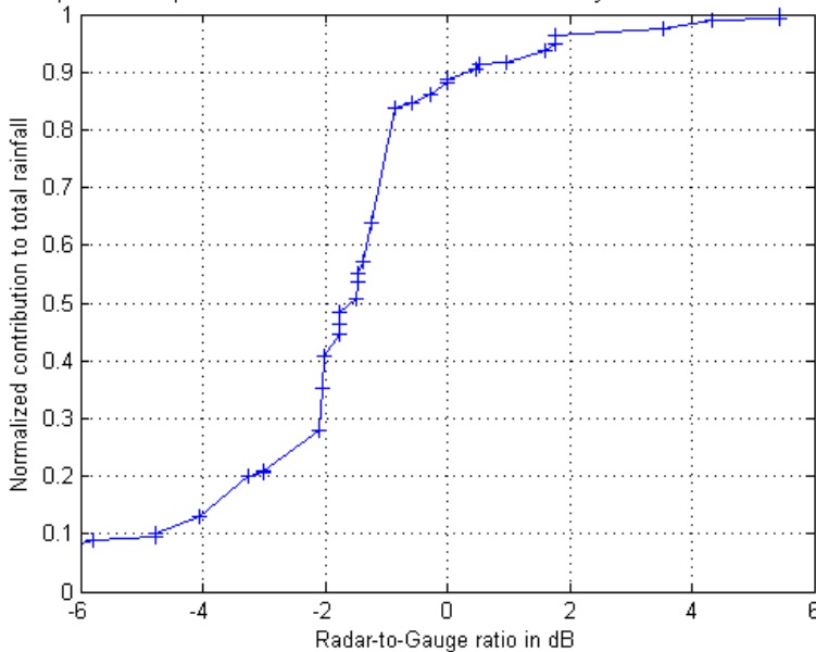
Fig. 12. As for Fig. 8, but for the 37 samples (G ≥ 0.4 mm/h) of the Giuliana rain gauge.
