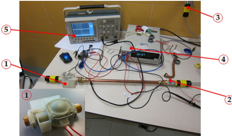
Figure 16. Wet Test Rig: scavenger (1), flow meter (2), domestic water supply and tap (3), multimeter (4) and oscilloscope (5).
