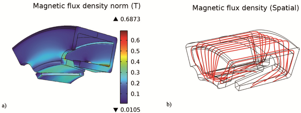
Figure 6. Results of the finite element simulations on the claw pole generator. a) Magnetic flux density in the stator in teslas (T); b) magnetic flux lines inside the iron.
