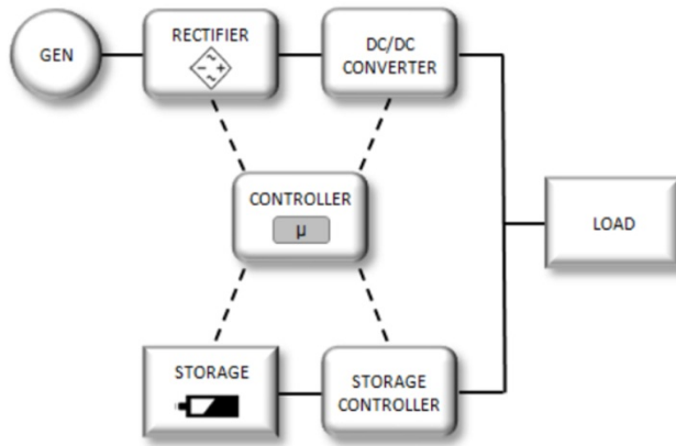
Figure 8. Architecture component interaction and interconnection.
