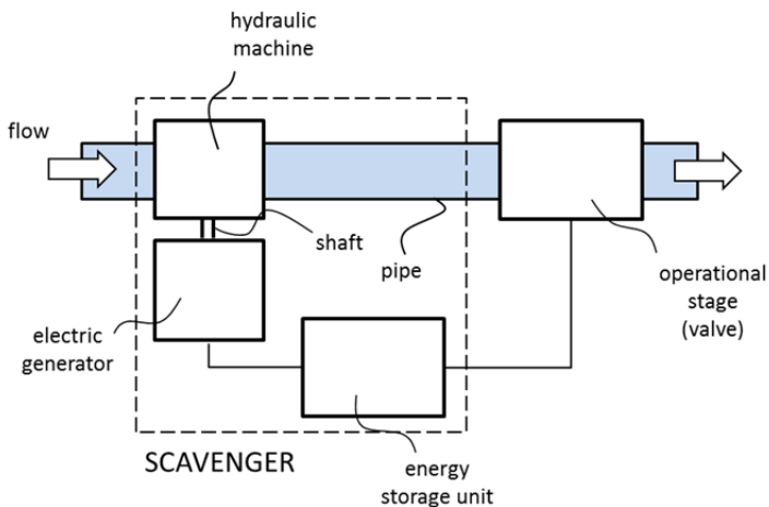
Figure 1. Hydraulic Energy Harvester system scheme
