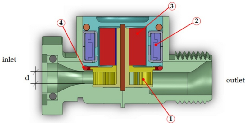
Figure 17. Cross-section view of the scavenger: Banki turbine (1), claw pole generator (2), permanent magnet rotor (3) and O-ring (4).
