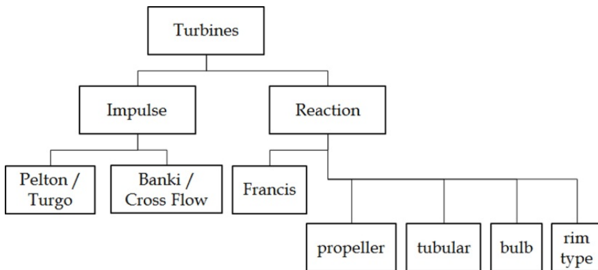
Figure 2. Classification of turbines for micro-hydropower generation
