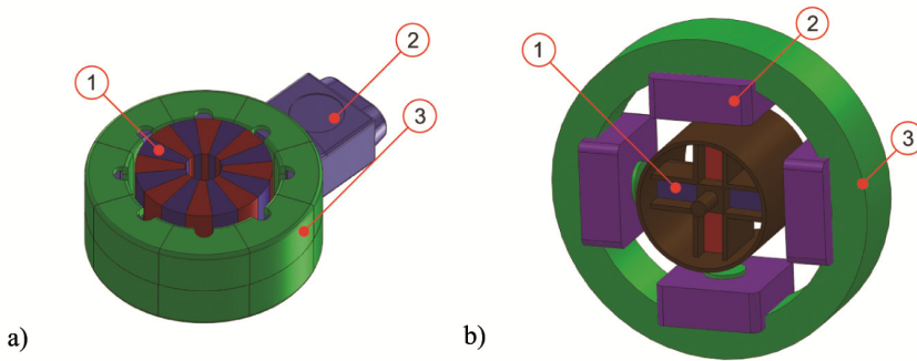
Figure 4. Configurations of electrical machines studied during the trade-off analysis. a) Two phase generator; b) Claw pole generator.
