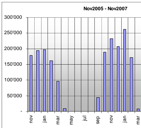
Electricity [MWh/month]
