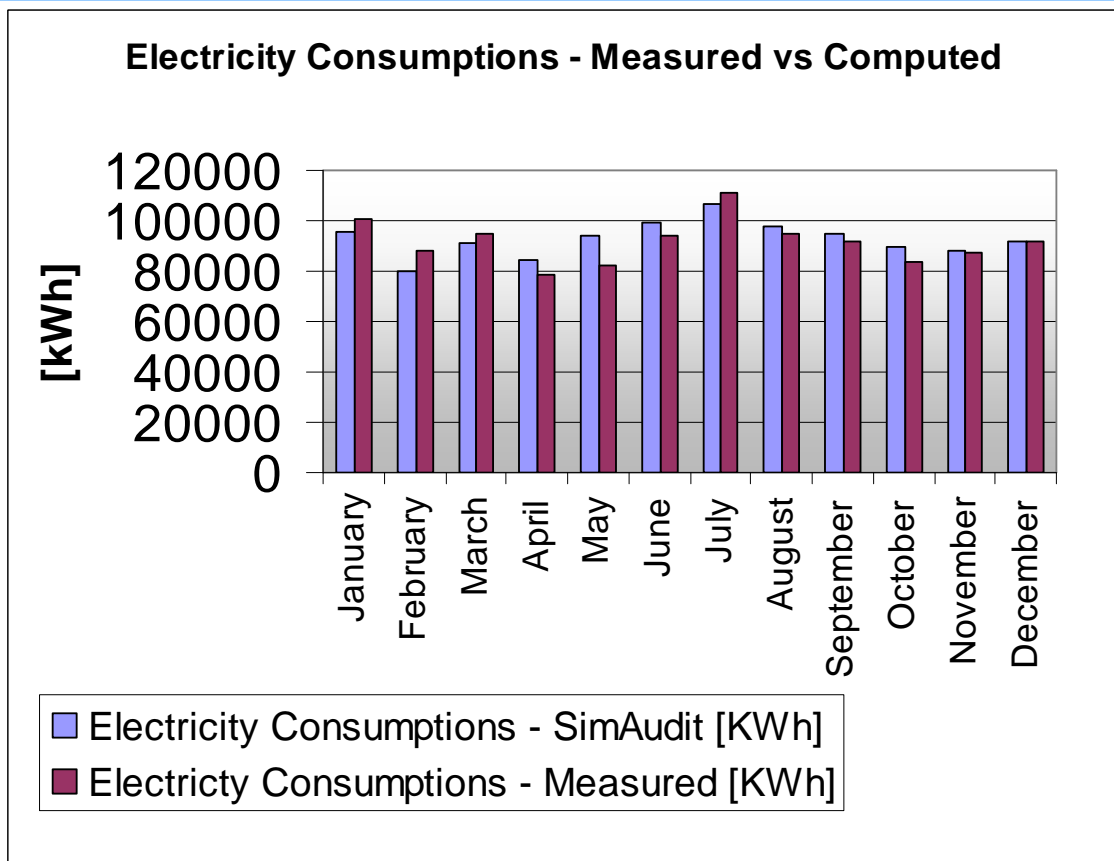
SimAudit Simulation
