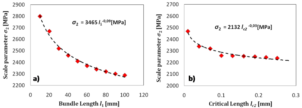
Fig. 2.8 Variation of the scale parameter \sigma_2 of the bundle at the second hierarchical level as a function a) of its length and b) of its critical length.
