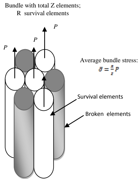
Fig. 3.2 Stress condition of the bundle.
