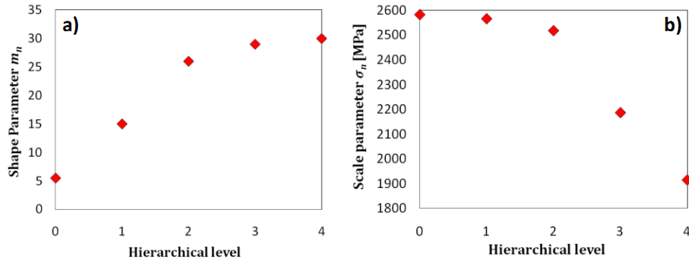
Fig. 2.10 Variation of shape parameter (a) and the scale parameter (b) as a function of the hierarchal level.
