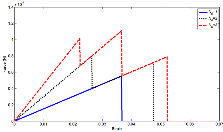
Fig. 4.9 Force-strain curves CNT bundle with for N_0=1 , N_0=2 and N_0=3 .
