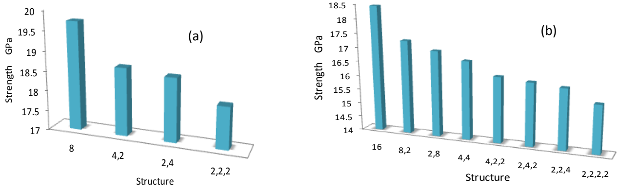
Fig. 5.7 Strength vs. Hierarchical level structure (a) N=8 and (b) N=16 .
