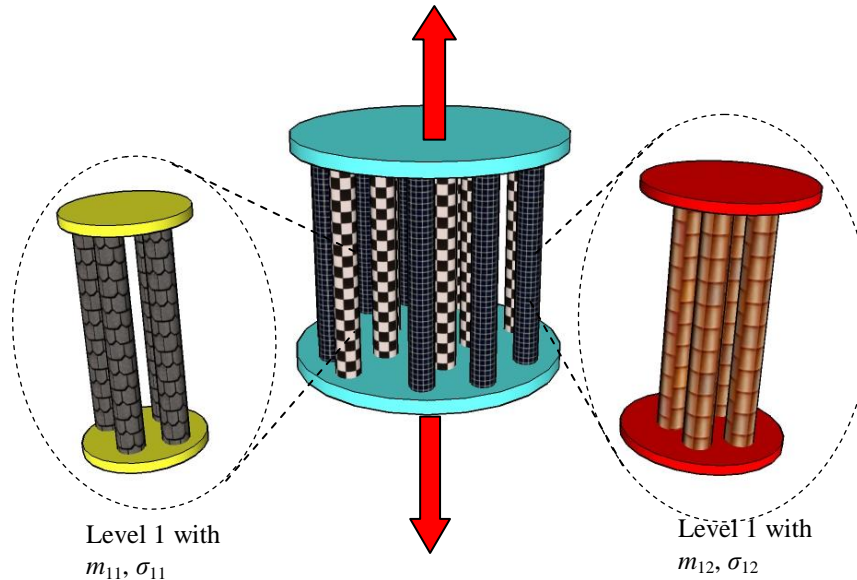
Fig. 5.19 Schematic of composite bundles of bundle.
