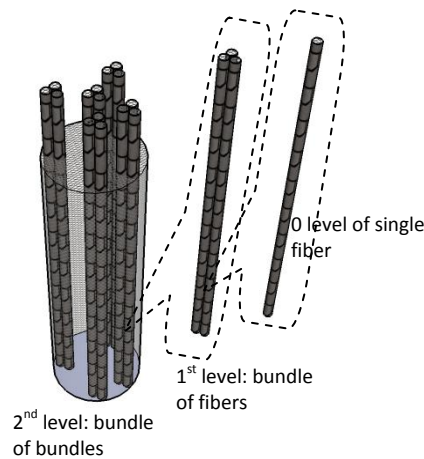
Fig. 5.5 Schematic of multi-scale (two levels) fiber bundle model.
