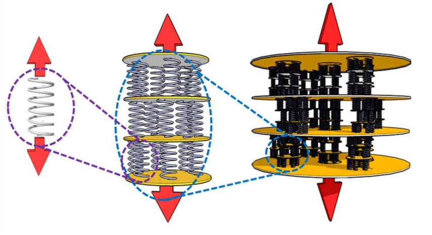
Fig. 2.5 Schematic representation of hierarchical procedure for chains of bundles
