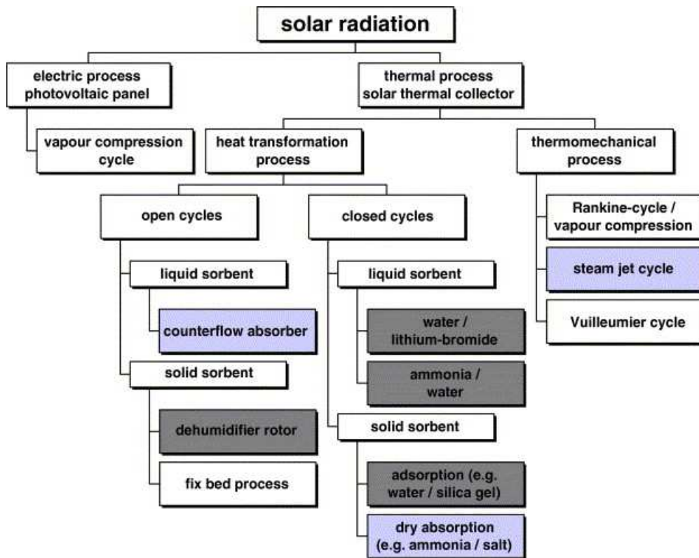
Figure 53 Physical ways to convert solar radiation into cooling or air-conditioning
