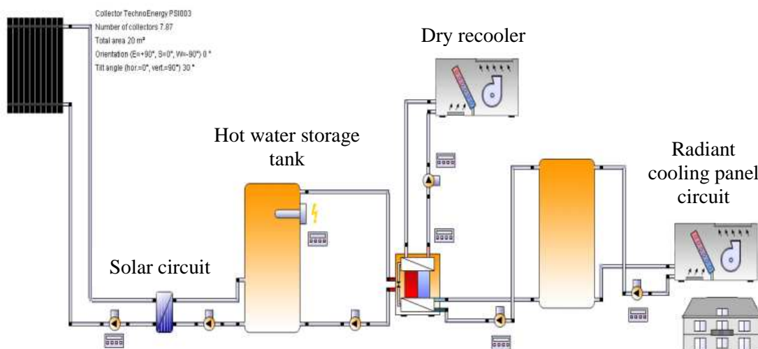
Figure 82 Scheme of the solar cooling system in PUEEL building
