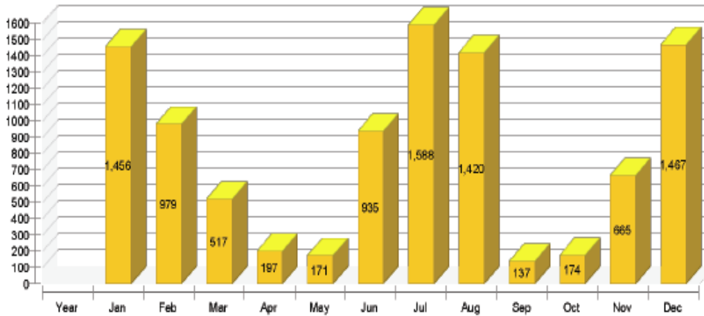
Figure 67 Heat generator energy to the system (solar thermal energy not included) for each month of year
