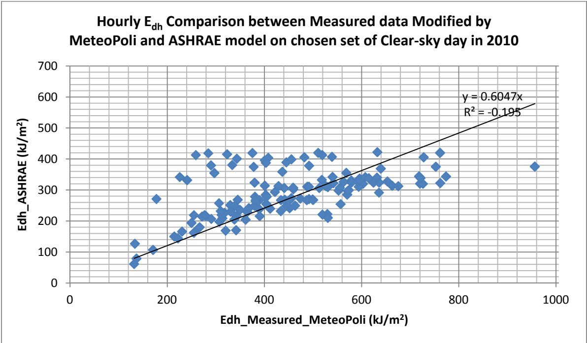
Figure 42 Hourly E_{dh} comparison between measured data in MeteoPoli and ASHRAE model on chosen set of clear-sky days in 2010
