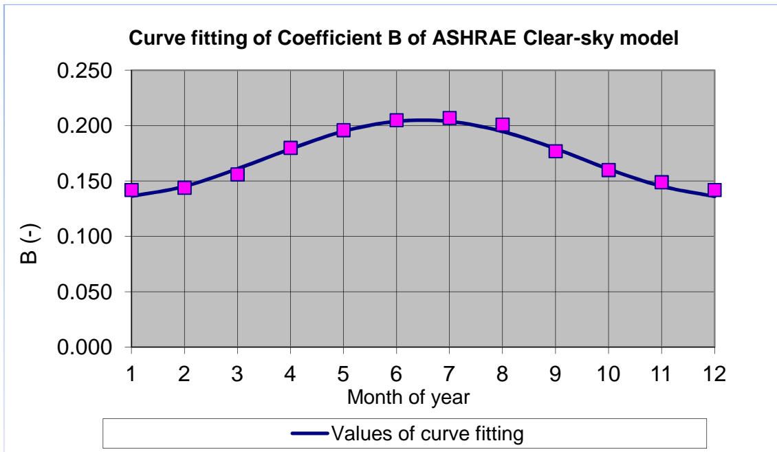
Figure 28 Curve fitting of coefficient B of ASHRAE Clear-sky model
