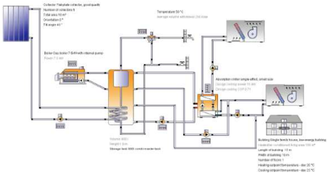
Figure 65 Schematic of template 71a - Space heating and cooling + hot water
