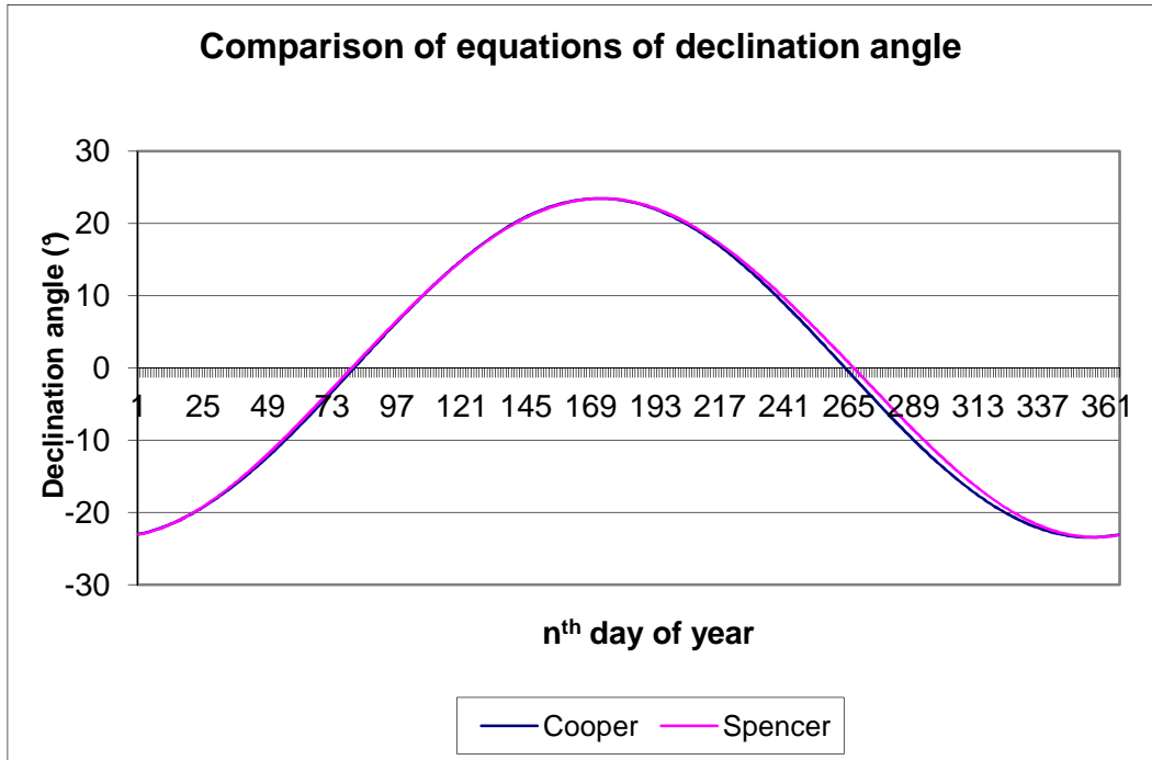
Figure 25 Comparison of equations of declination angle
