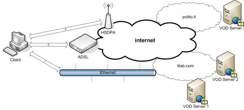
Fig. 3. Network topology
