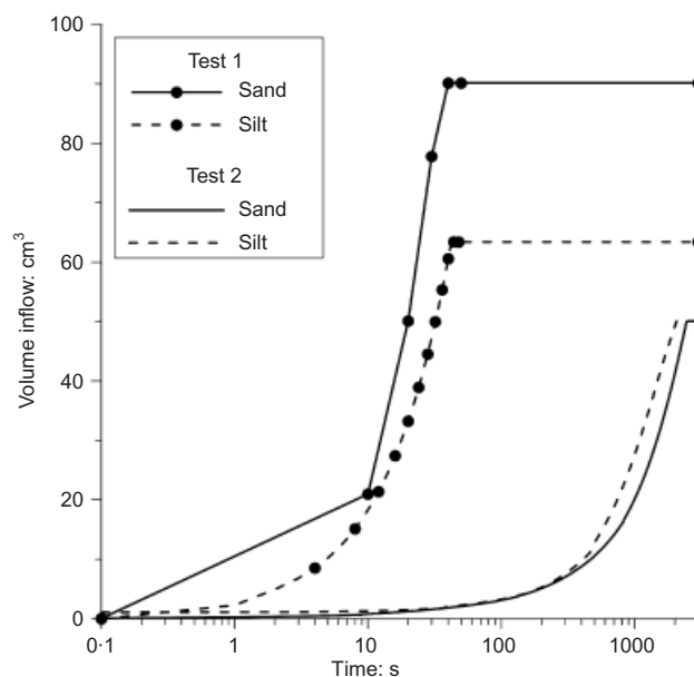
Fig. 6. Time evolution of water inflow for the performed tests
