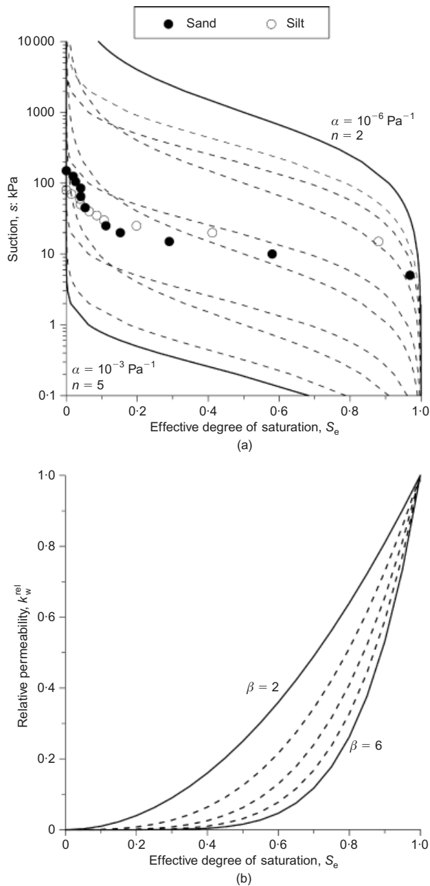
Fig. 12. Domain explored in terms of: (a) water retention curve; (b) relative permeability function. Continuous lines and points represent boundaries of explored space and independent axis-translation data respectively
