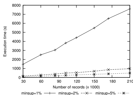
Figure 4.21: GENIO: scalability on TPC-H datasets
