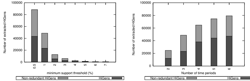
(a) Impact of the support threshold. Time periods=3. Taxonomy height=3
