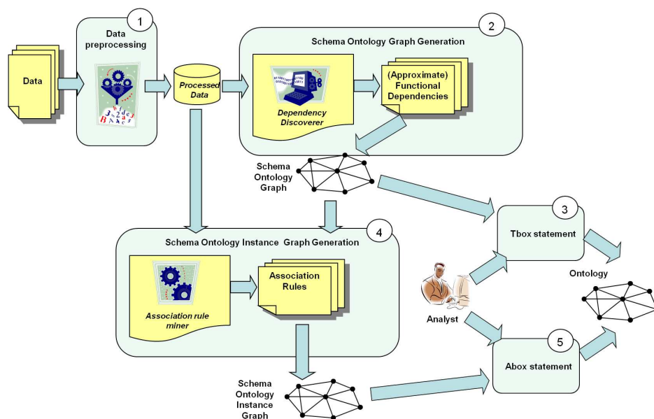
Figure 7.3: The DONG framework architecture.
