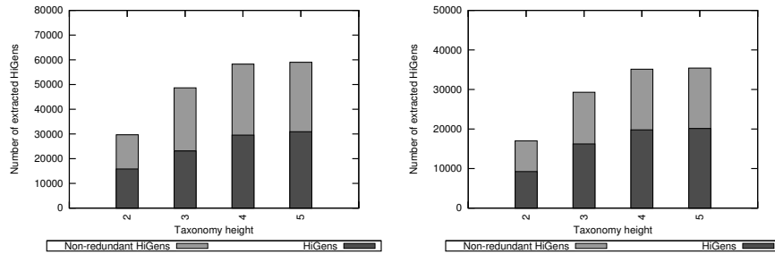
(c) Impact of the taxonomy height. Equi-depth discretization. min\_sup=1\% . Time periods=3.
