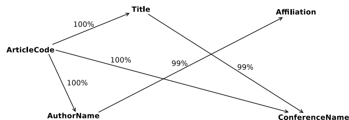
Figure 7.1: A simplified SONG built over the example DBLP XML attributes.
