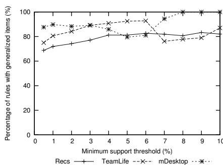
Figure 4.9: CAS-MINE: percentage of selected rules with generalized items by varying the minimum support threshold. \text{Minconf} = 0\%
