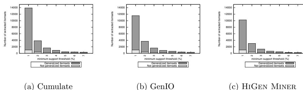
Figure 6.4: HiGEN MINER: generalized and not generalized itemsets extracted from data-3
