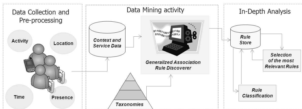
Figure 4.6: The CAS-MINE framework architecture
