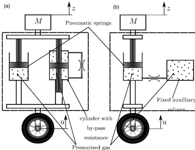
Figure 1. (a) BPR and (b) FAV suspension systems.
