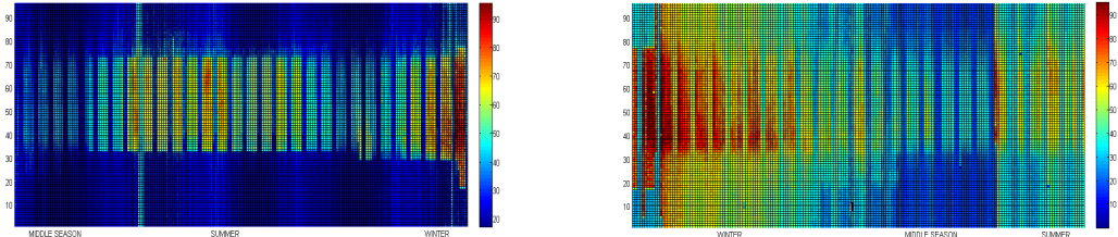
Figure 11. Carpet plots of total electric energy consumption with different VRF schedules
