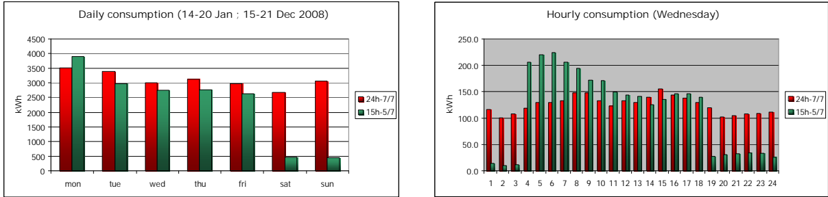
Figure 10. Daily and hourly electric energy demand of VRF system with different schedules
