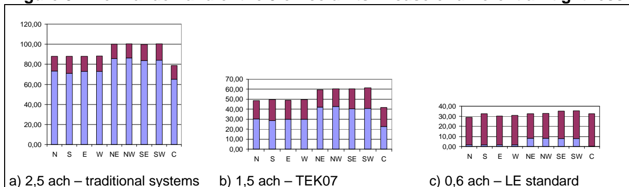
Figure 8. Thermal demand of the 9 office units in case of different air-tightness.
