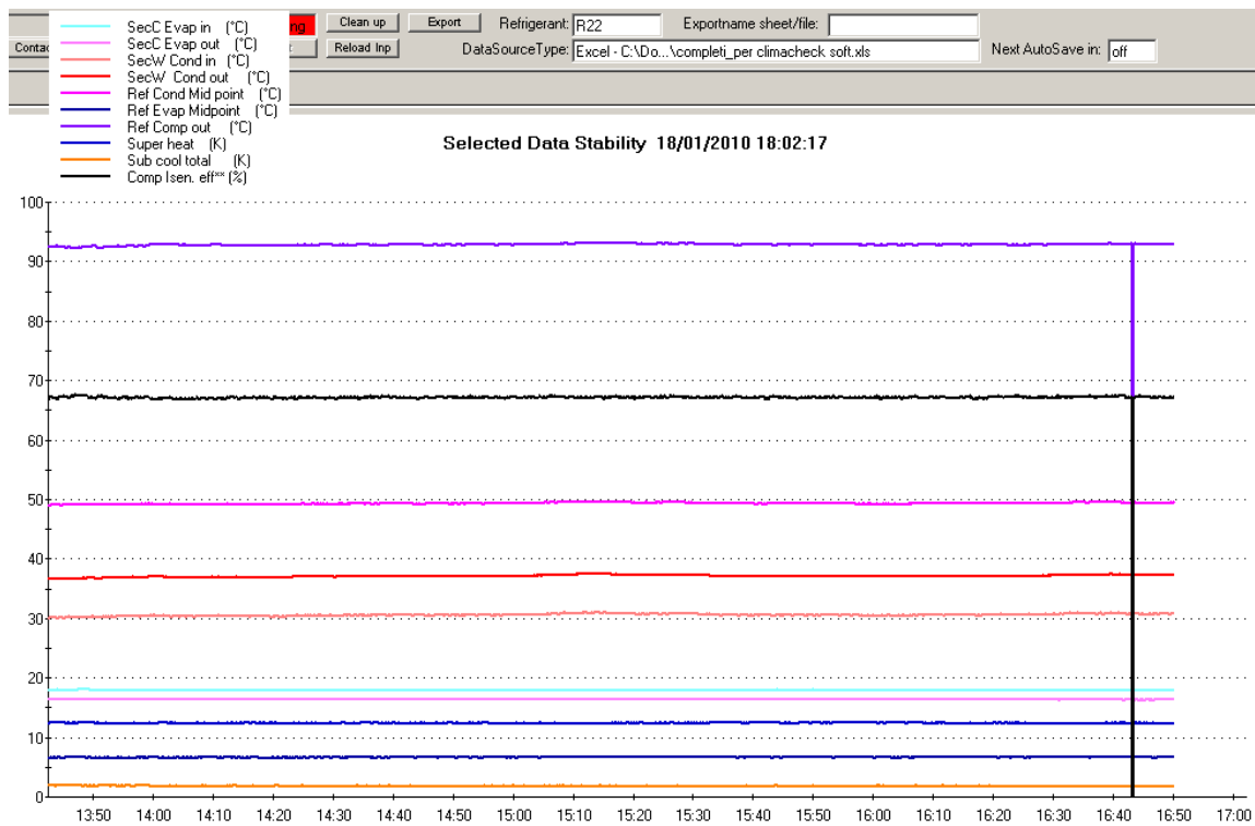
Figure 14. Case Study 5: Chiller parameters logged
