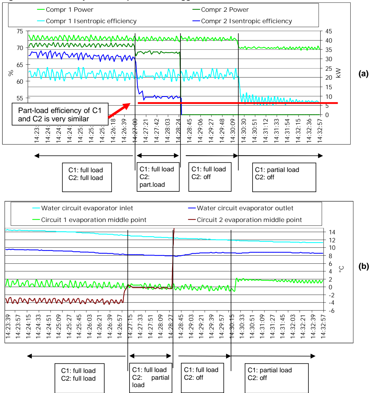
Figure 13. Case Study 4: Chiller parameters logged
