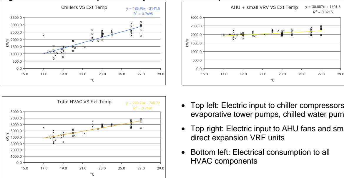
Figure 2. Electric consumption vs daily mean external temperature for different users
