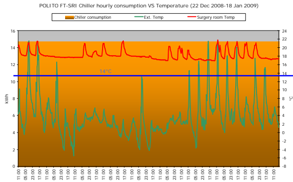
Figure 8. Outdoor / indoor temperature - chiller electric consumption (December – January)
