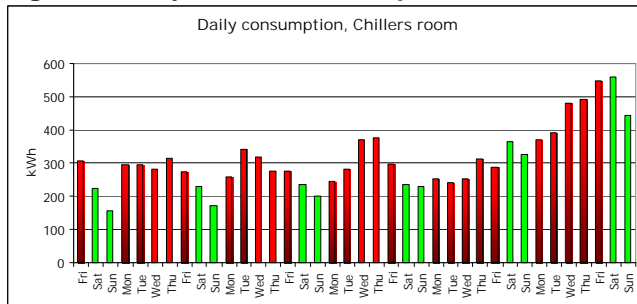
Figure 9. Daily electric consumption of central cooling plant: workdays and weekends
