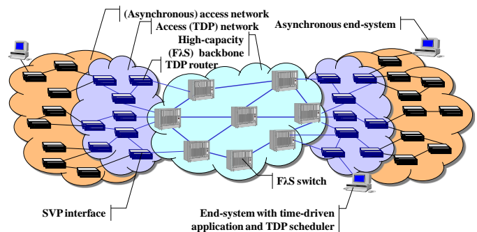
Figure 3. Architecture for deploying pipeline forwarding
