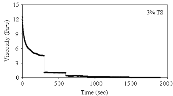
Fig. 8a: Step-test results (3% TS sludge with polyelectrolyte)
