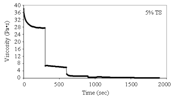
Fig. 8b: Step-test results (5% TS sludge with polyelectrolyte)
