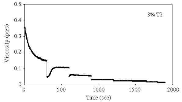
Fig. 7a: Step-test results (3% TS sludge without polyelectrolyte)
