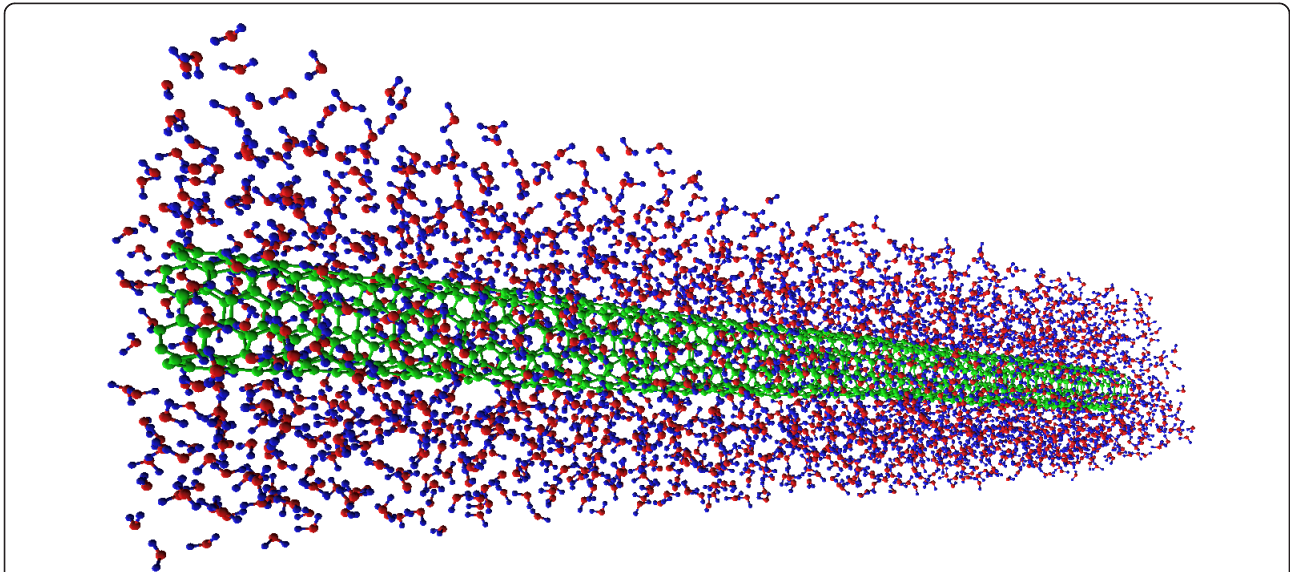
Figure 6 Color online. A (5, 5) SWCNT (green) is surrounded by water molecules (blue, red). Nosé-Hoover thermostats with temperature T_{hot} = 360 K are coupled to the nanotube tips, while water is kept at a fixed temperature T_w = 300 K. After a sufficiently long time (here 15 ns), a steady-state condition is reached. MD simulation results (in terms of both temperature profile and heat flux) are consistent with a continuous one-dimensional model as described by Equations (17) and (18). Image obtained using VEGA ZZ [47].
