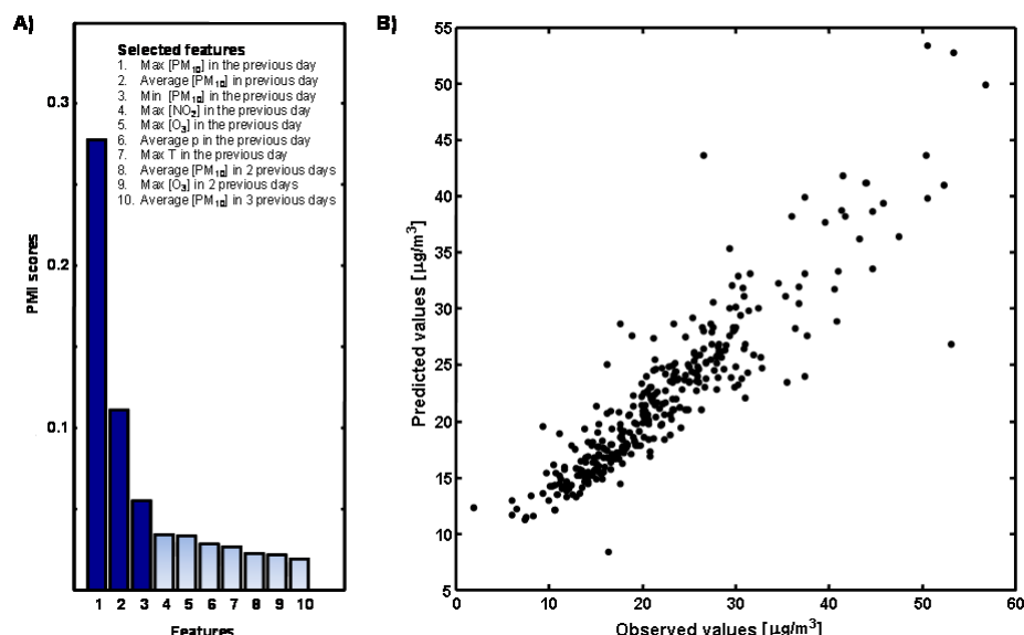
Fig. 1. A) Partial mutual information scores for the 10 most significant features. The first three features were selected by the Hampel test. B) Comparison between the observed and predicted \text{PM}_{10} concentration.
