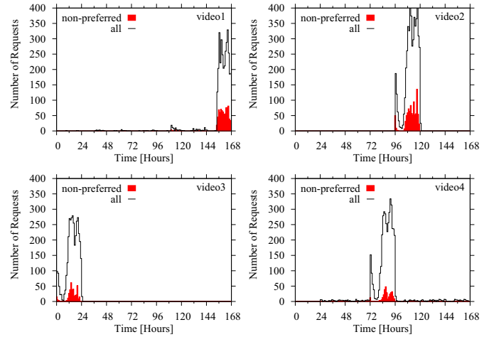
Fig. 14. Load related to the top 4 videos with the highest number of accesses to the non-preferred data centers for the EU1-ADSL dataset.
