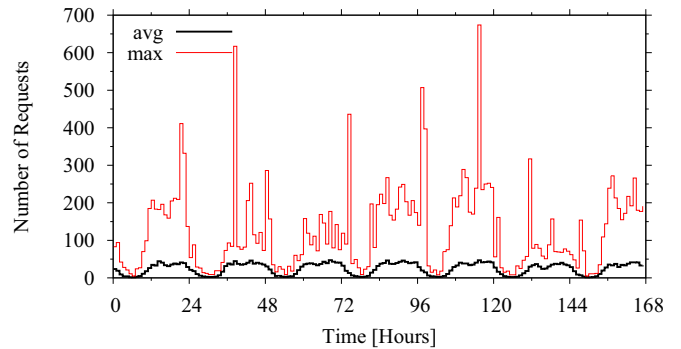
Fig. 15. Average and maximum number of requests per server in the preferred data center of EU1-ADSL dataset.
