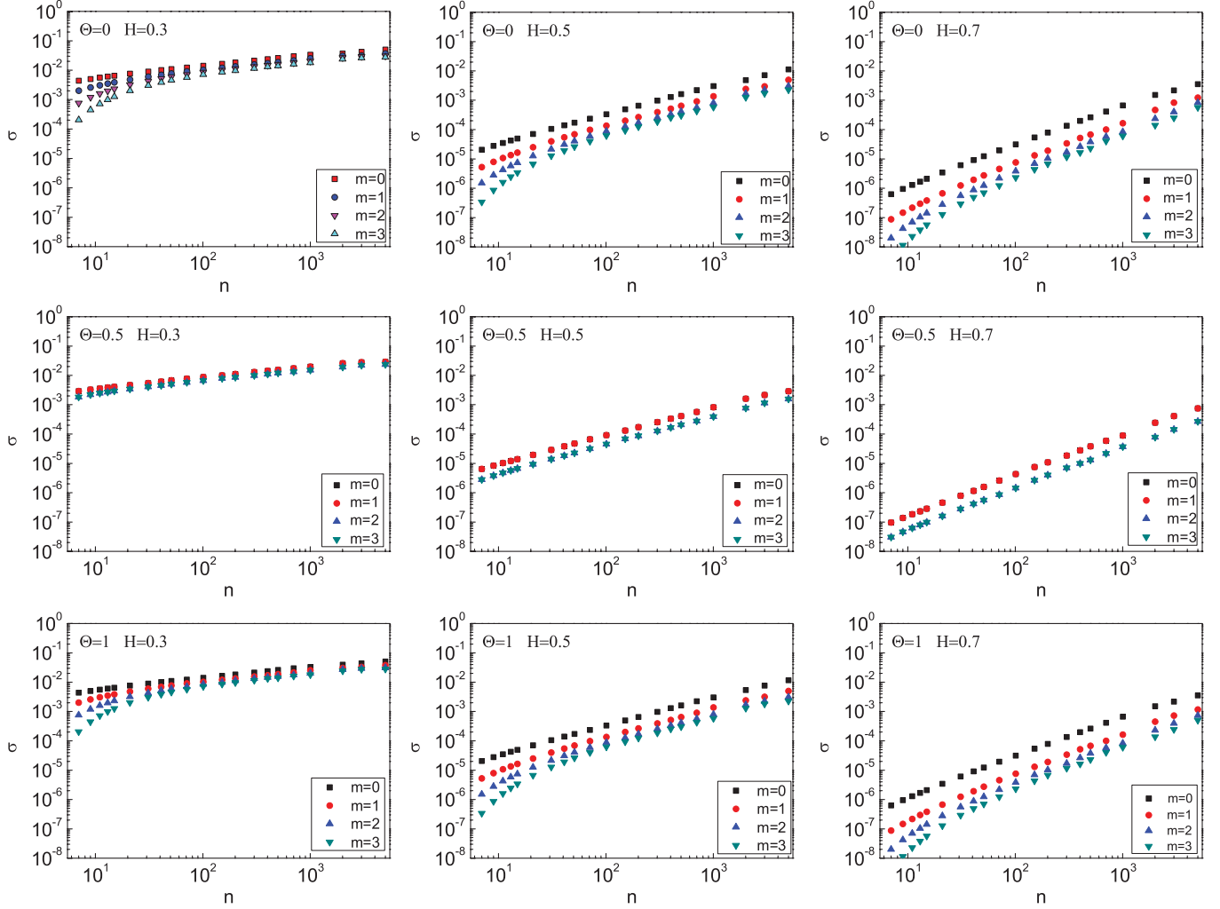
FIG. 2. (Color online) Log-log plots of \sigma_{DMA}^2 vs n for moving average polynomial degree m = 0 , m = 1 , m = 2 , and m = 3 , referred, respectively, to the endpoints ( \theta = 1 ; \theta = 0 ) and to the midpoint ( \theta = 0.5 ) of the window n . The series have been generated by the random midpoint displacement algorithm. The nominal Hurst exponent is H = 0.3 , H = 0.5 , and H = 0.7 . The values of H obtained on five samples of such series are shown in Table I.
