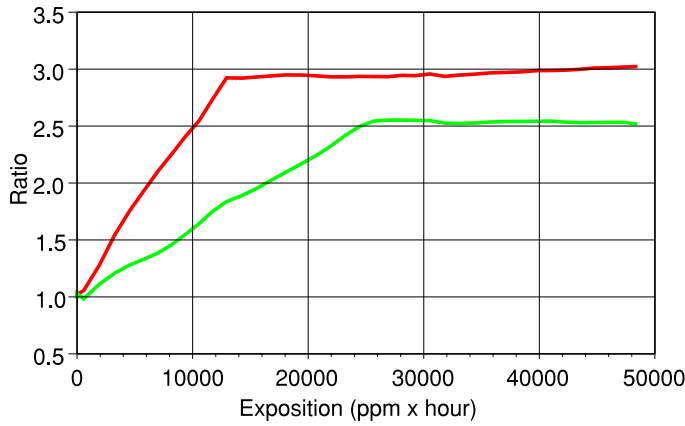
Fig. 7. Attenuation change as a function of the HF vapor exposition the two different fibers whose FTIR is shown in fig 6. The red line refers to the fiber obtained with an oxygen rich plasma and which has a SiO_2 -like coating. The exposition is computed by integrating the partial pressure computed according to eqn. 2
