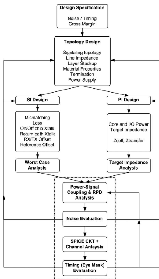
Fig. 2. Design flow.
