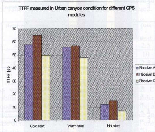
Fig.24: TTFF evaluated in an urban canyon environment through different GPS receivers.
