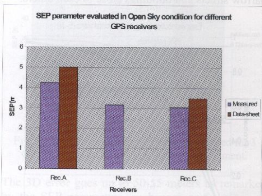
Fig.8-9: CEP and SEP parameters evaluated for different GPS modules and in an open sky environment.
