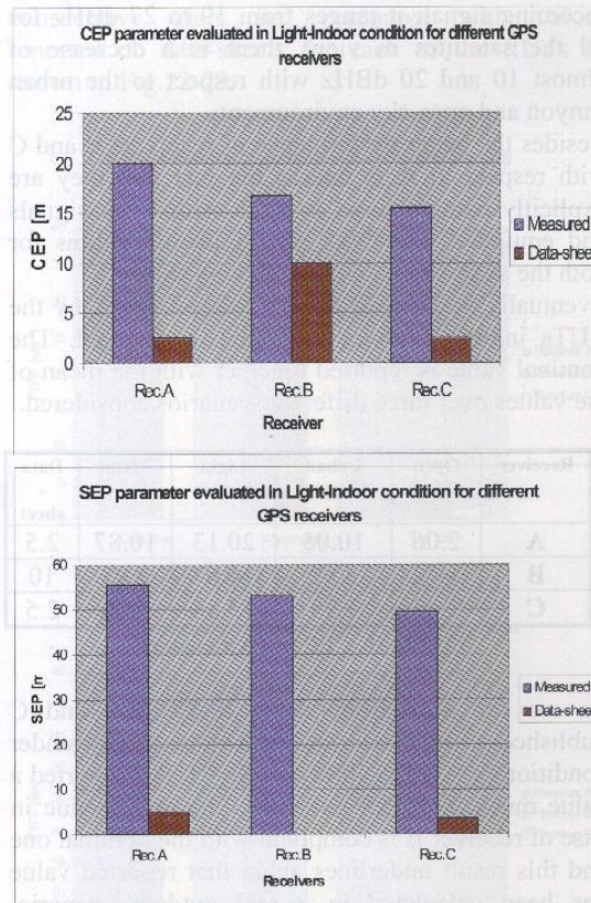
Fig.16-17: CEP and SEP parameters evaluated for 3 GPS modules and in a Light Indoor environment.
