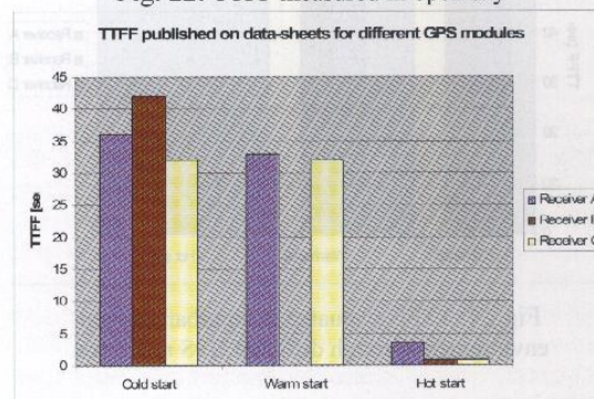
Fig. 22-23: TTFF as reported on data-sheet
