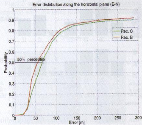
Fig.19: Error Distribution on the horizontal plane for different GPS modules in Deep Indoor condition
