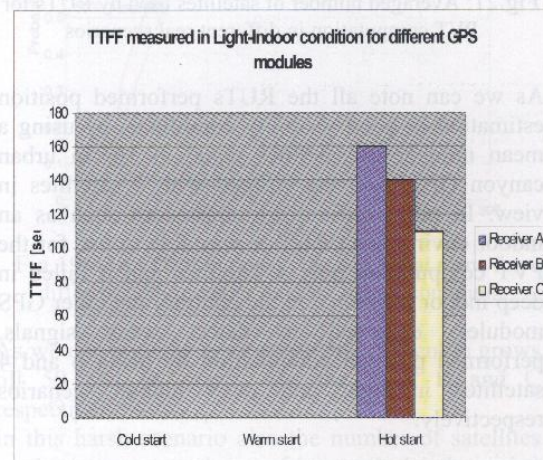
Fig.25: TTFF evaluated in a light indoor environment through different GPS receivers.
