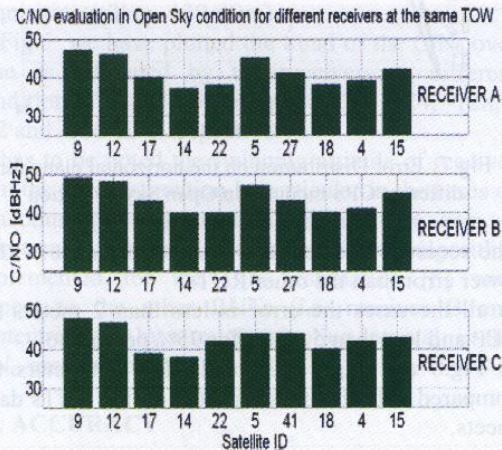
Fig.10: C/N_0 evaluated for each satellite in view at the same TOW by different mass- market receivers
