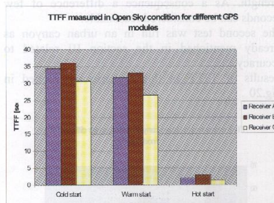
Fig. 22: TTFF measured in open sky
