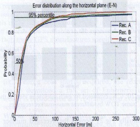
Fig. 15: Error Distribution on the horizontal plane for different GPS modules in Light Indoor condition
