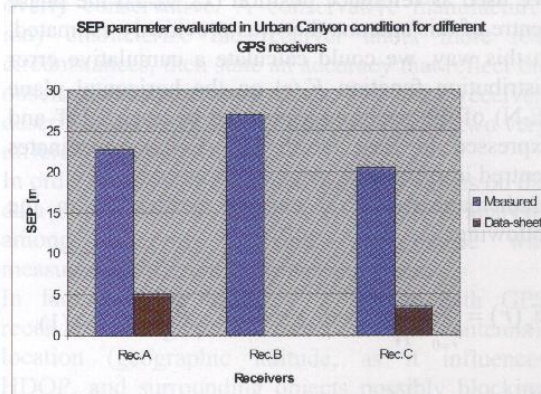
Fig.12-13: CEP and SEP parameters evaluated for different GPS modules in an Urban Canyon environment.
