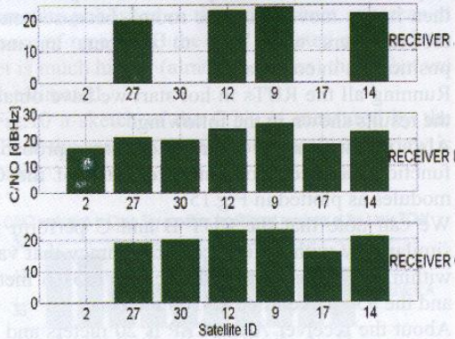
Fig.18: C/N 0 evaluated for each satellite in view at the same TOW by different mass-market receivers
