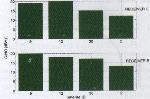
Fig.20: C/N 0 evaluated for each satellite in view at the same TOW by different mass-market receivers
