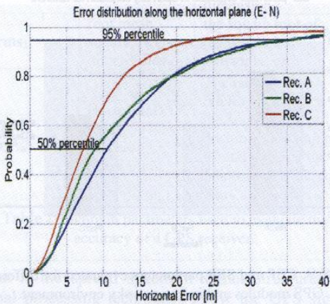
Fig.11: Error Distribution on the horizontal plane for different GPS modules in urban canyon condition
