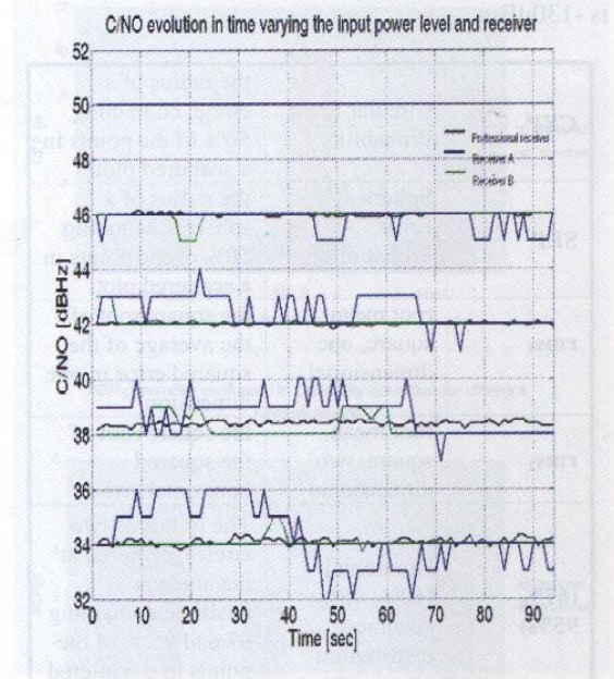
Fig.5: C/N_0 estimation varying with time and with the input power level evaluated for different GPS receivers
