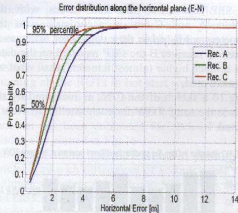
Fig.7: Error Distribution on the horizontal plane for different GPS modules in Open Sky condition
