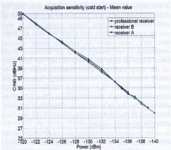
Fig.3: Mean values of the C/N_0 for the Acquisition sensitivity evaluation working with different GPS modules
