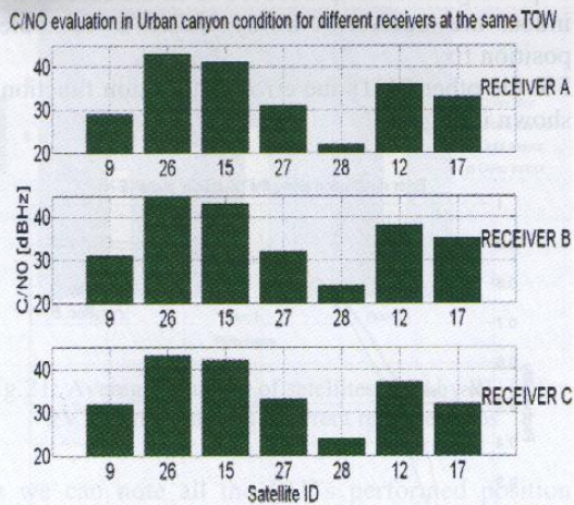
Fig. 14: C/N 0 evaluated for each satellite in view at the same TOW by different mass- market receivers
