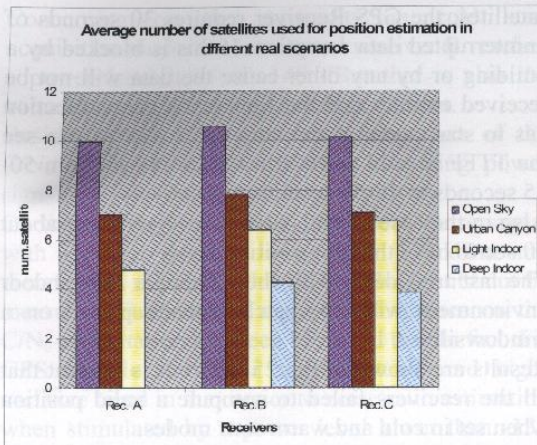
Fig.21: Averaged number of satellites used by RUTs for PVT computation in different real scenarios
