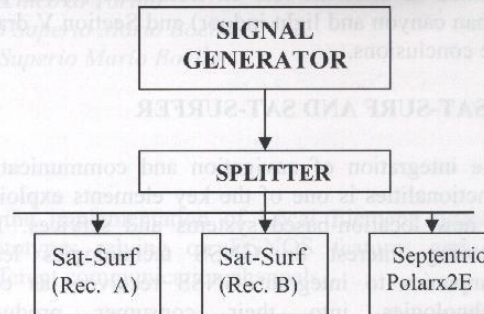
Fig.2 Setup used for the sensitivity receiver analysis
