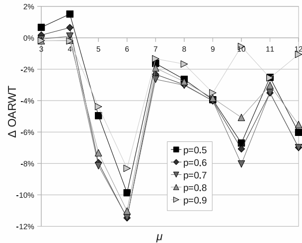
Figure 10: difference between the OARWT provided by DCS and PDCS with various p , with AN = 9.94 , NV = 9.41 , and random deployment
