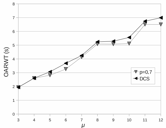
Figure 11: OARWT provided by DCS and PDCS ( p = 0.7 ) with AN = 9.94 , NV = 9.41 , and random deployment
