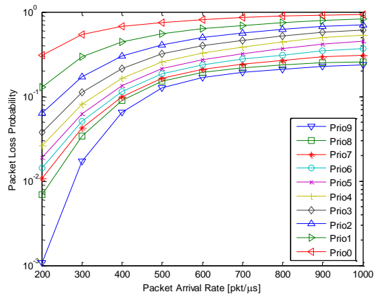
Fig. 14. Packet loss probability versus packet arrival rate for M = 10 .
