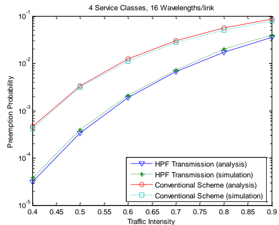
Fig. 4. Preemption probability at a single OBS output port ( W = 16, M = 4 ).
