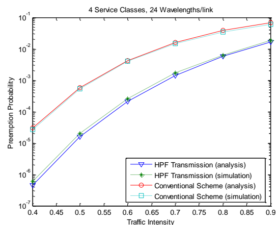
Fig. 5. Preemption probability at a single OBS output port ( W = 24, M = 4 ).
