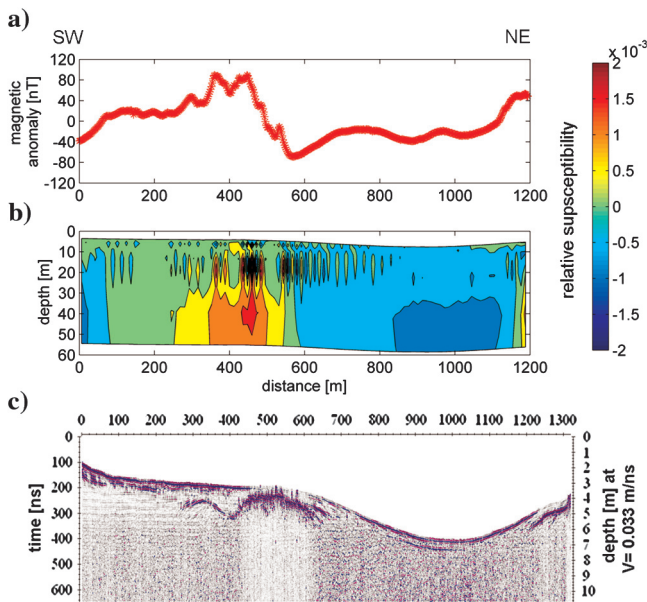
Figure 15. (a) magnetic anomaly and (b) relative susceptibility contour map produced by the 2D inversion of magnetic profile 20, and (c) GPR bathymetry profile.
