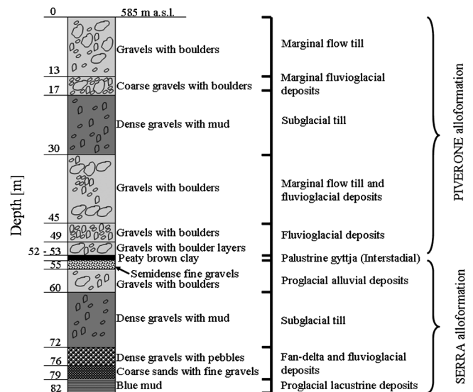
Figure 2. Stratigraphic log of the geological environment.
