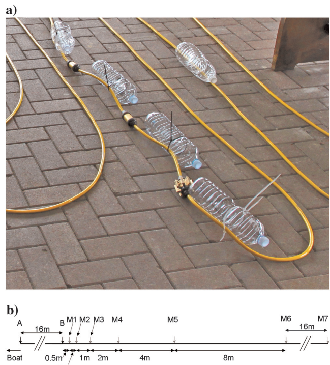
Figure 4. Electrical cable: (a) a current electrode with radial fins and cylindrical potential electrodes. Empty bottles kept the cable floating; (b) electrodes geometry.
