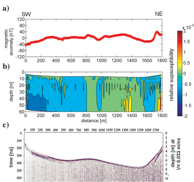
Figure 13. (a) magnetic anomaly and (b) relative susceptibility contour map produced by the 2D inversion of magnetic profile 15, and (c) GPR bathymetry profile.
