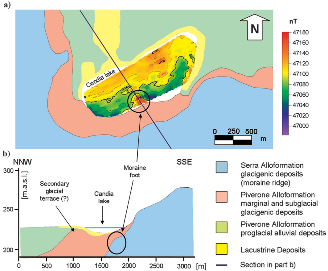
Figure 12. Geological setting of the area: (a) magnetic field strength superimposed upon the geologic map (modified after Gianotti et al., 2008) and (b) geological section cutting the main magnetic anomaly.
