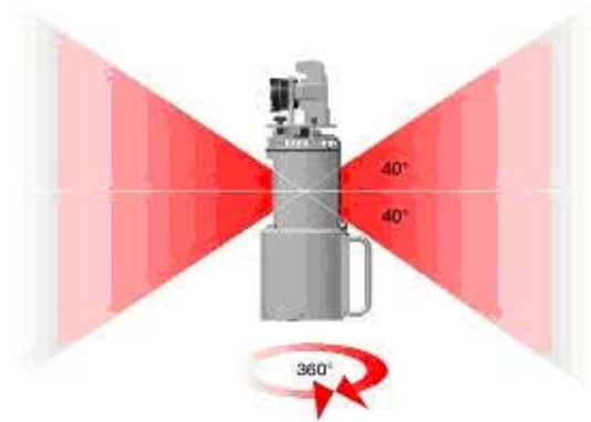
Fig. 2 – The Riegl LMS-Z420i laser field of view.
