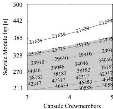
Fig. 12. Capsule and service module assembly mass [kg], as a function of the service module propellant I_{sp} and number of crewmembers hosted in the capsule. The other parameter levels are as follows A_{Level-1} , B_{Level-1} , D_{Level1} , E_{Level0} , F_{Level0} , H_{Level0} .
