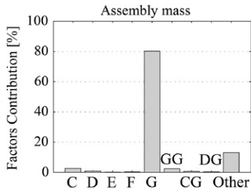
Fig. 7. Factors' contribution to the mass of Capsule plus Service module.
