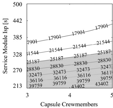
Fig. 11. Capsule and service module assembly mass [kg], as a function of the service module propellant I_{sp} and number of crewmembers hosted in the capsule. The other parameter levels are as follows A_{Level-1} , B_{Level-1} , D_{Level-1} , E_{Level0} , F_{Level0} , H_{Level0} .
