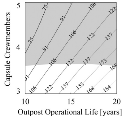
Fig. 9. Number of launches as a function of the outpost operational life and number of capsule crewmembers. The other parameter levels are as follows A_{Level-1} , D_{Level1} , E_{Level-1} , F_{Level0} , G_{Level0} , H_{Level0} . The grey area is infeasible.
