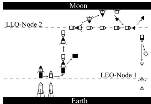
Fig. 1. Schematic of the reference mission architecture.
