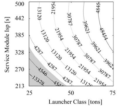
Fig. 13. Constraint as a function of the launcher class and service module propellant I_{sp} . The other parameter levels are as follows B_{Level0} , C_{Level0} , D_{Level0} , E_{Level0} , F_{Level0} , H_{Level0} .
