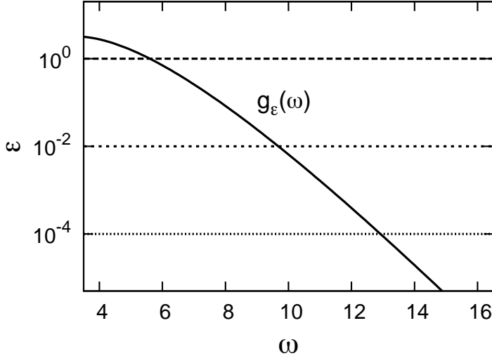
Figure 8: Plot in lin-log scale of the function g_\epsilon(\omega, 1, 1) , see equation (22), which qualitatively defines the thermodynamic regime of the solution.
