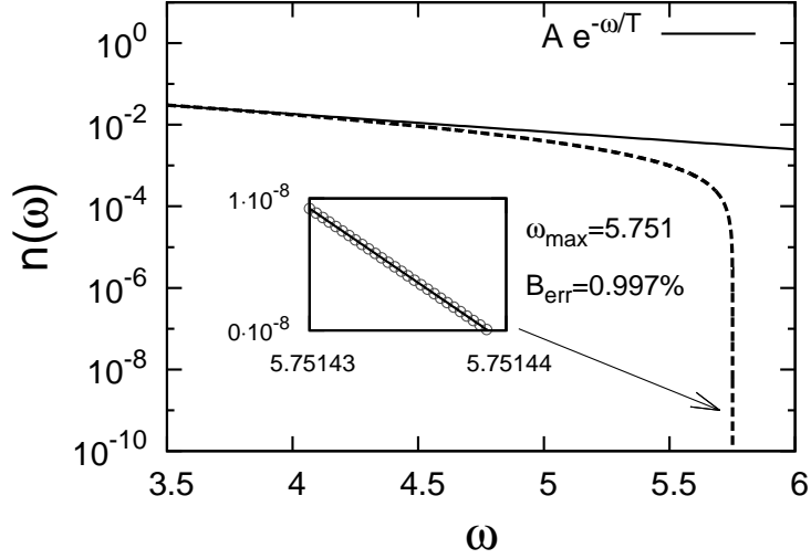
Figure 9: DAM simulation of ODE- \epsilon (16) with constant energy flux \epsilon = 1 (dashed line). The initial conditions in \omega_0 = 3.5 are set by the MB distribution with T = 1 and A = 1 (continuous line). The inset shows a zoom of numerical n(\omega) (dots) in the vicinity of the point \omega_{\max} where a linear fit is shown by continuous line.
