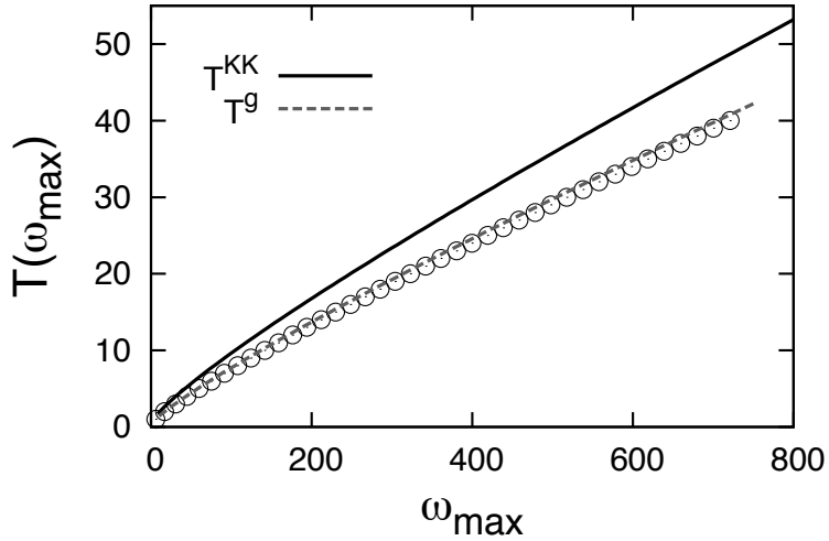
Figure 10: Checking of predictions in DAM constant energy flux cascade (16): the points represent the temperature of the initial condition T with respect to the measured \omega_{\max} . Solid line is the matching relation (20) while dashed one is obtained from (23).
