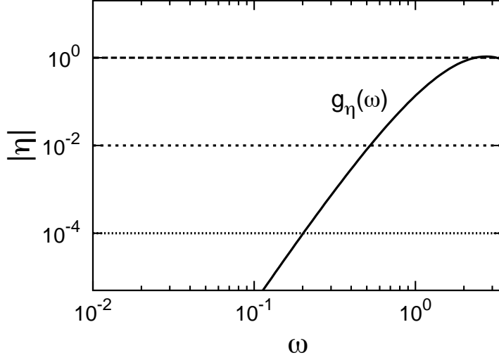
Figure 12: Plot of the function g_\eta(\omega, 1, 1) , see equation (30).
