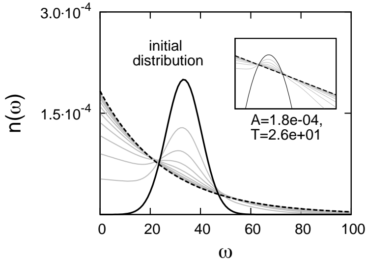
Figure 1: Numerical computation of HIBE with an initial Gaussian shaped distribution (continuous black line): intermediate states are shown with gray lines and final steady distribution with dashed black line. The latter has a MB behavior (7) with fitted parameters A and T printed in figure. The inset shows the same plot in lin-log scale.
