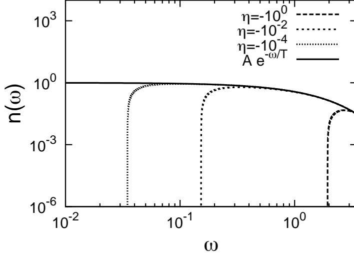
Figure 11: DAM simulations of (25) for different constant inverse particle flux \eta starting with the same initial condition at \omega_0 = 3.5 given by the Boltzmann distribution n_{MB}(\omega) = Ae^{-\frac{\omega}{T}} where A = 1 and T = 1 (plotted with continuous line).
