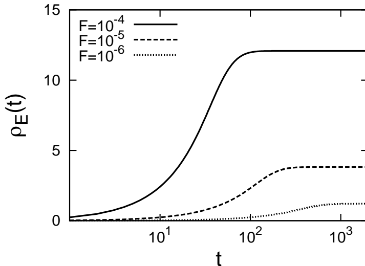
Figure 5: Total energy densities \rho_E(t) in function of time for different forcing rates F . For the system parameters refer to ones in Fig. 4.
