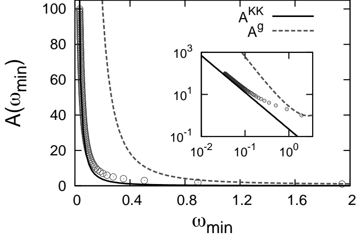
Figure 14: Checking predictions in DAM constant inverse flux cascade (25): the points represent the thermodynamic quantity A with respect to the measured \omega_{\min} . Continuous line is the KK matching prediction given in equation (28) while dashed one is obtained from (31).
