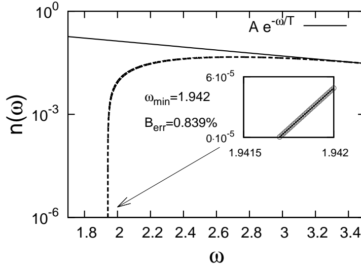
Figure 13: DAM simulation of (25) with \eta = -1 (dashed line) starting with initial condition at \omega_0 = 3.5 given by the MB distribution n_{MB}(\omega) = A e^{-\frac{\omega}{T}} where A = 1 and T = 1 (plotted with continuous line). Inset: lin-lin scale zoom in the vicinity \omega_{\min} (dots) where the best linear fit is presented with a continuous line.
