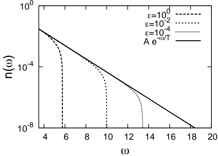
Figure 7: DAM simulations of (16) for different constant energy flux \epsilon starting with the same initial condition at \omega_0 = 3.5 given by the MB distribution n_{MB}(\omega) = A e^{-\frac{\omega}{T}} where A = 1 and T = 1 (continuous line).
