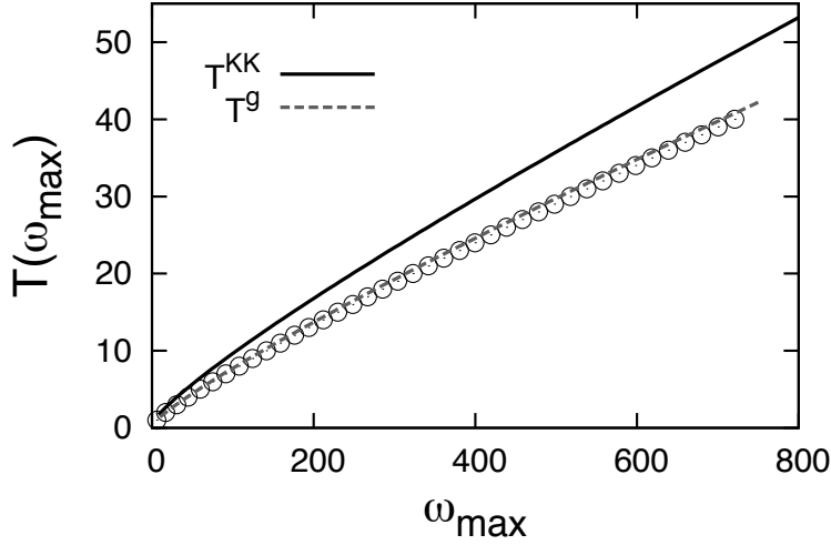
Figure 10: Checking of predictions in DAM constant energy flux cascade (16): the points represent the temperature of the initial condition T with respect to the measured \omega_{\max} . Solid line is the matching relation (20) while dashed one is obtained from (23).
