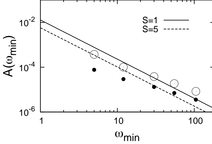
Figure 20: Thermodynamic amplitude A for different \omega_{\min} and fixed forcing in log-log scales in numerical simulations of HIBE. Filled circles corresponds to A_L while empty circles to A_R . The continuous and dashed lines are formula (32) with S = 1 and S = 5 respectively.
