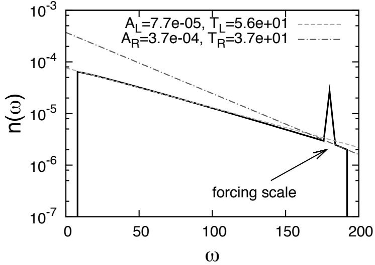
Figure 3: An example of HIBE (9) steady state shown with black line in lin-log scale. Simulation parameters are: \omega_{\min} = 5 , \omega_f = 182 , \omega_{\max} = 195 and F = 10^{-5} , and \omega_{cutoff} = 200 . The dashed and point/dashed lines are left and right branch best fits obtained with the MB distribution (7): fitting parameters are reported in label.
