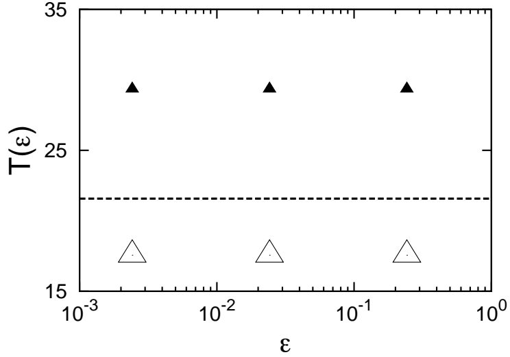
Figure 17: Measured temperatures T_L (filled triangles) and T_R (empty ones) obtained in the simulations shown in Fig. 4. The dashed line is the analytical prediction (32).
