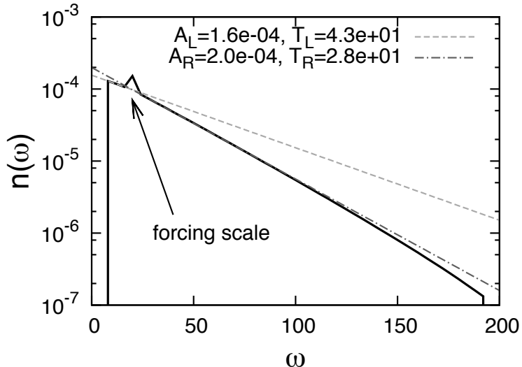
Figure 2: An example of HIBE (9) steady state shown with black line in lin-log scale. Simulation parameters are: \omega_{\min} = 5 , \omega_f = 22 , \omega_{\max} = 195 and F = 10^{-5} , and \omega_{cutoff} = 200 . The dashed and point/dashed lines are left and right branch best fits obtained with the MB distribution (7): fitting parameters are reported in label.
