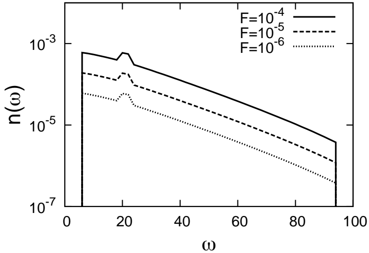
Figure 4: Steady states of HIBE (9) in lin-log scale obtained for different values of the forcing rate F . Parameters are \omega_{cutoff} = 200 , \omega_{\min} = 5 , \omega_f = 21 and \omega_{\max} = 95 .
