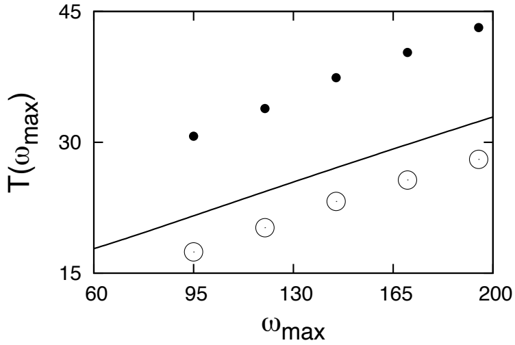
Figure 18: Temperature in different steady state keeping the forcing constant and varying the dissipation scale \omega_{\max} : big empty circles correspond to the temperature T_R on the right of the forcing scale, whereas small filled circles to the left side, T_L . The continuous line is the prediction (32).
