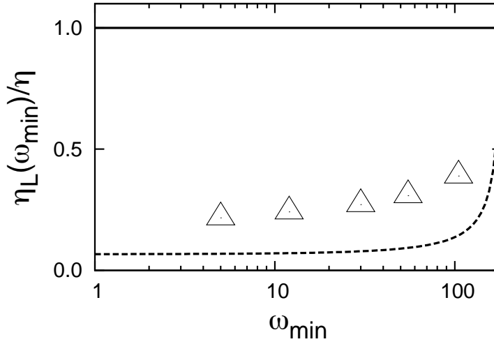
Figure 21: The plot shows in log-linear scale the ratio of the measured inverse particle flux over the total one \eta_L/\eta (empty triangles) with respect to \omega_{\min} ; the continuous line correspond to the total flux while the dashed one follows the finite range correction (34).
