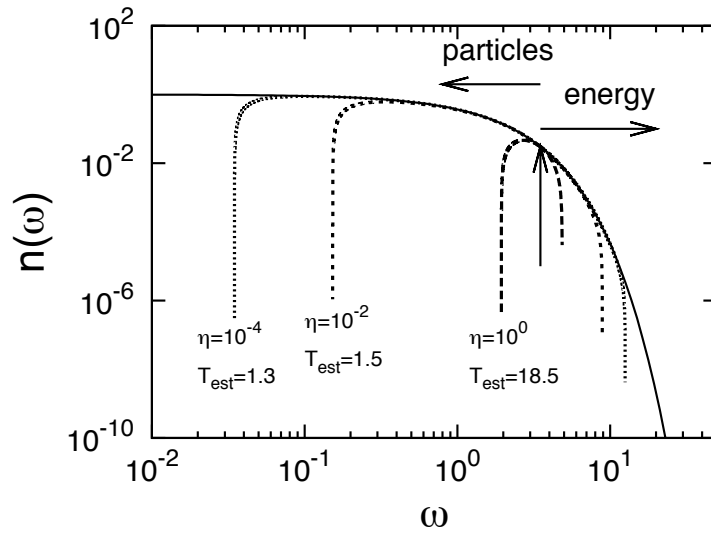
Figure 15: DAM double cascade simulations of equations (16) and (25) for three different values of the particle flux \eta (and consequently of the energy flux \epsilon = \eta \omega_f ). The initial condition are taken at \omega_f = 3.5 from the MB distribution with T = 1 and A = 1 . Measuring \omega_{\min} and \omega_{\max} in each case we estimate of the temperature T_{est} from prediction (32).
