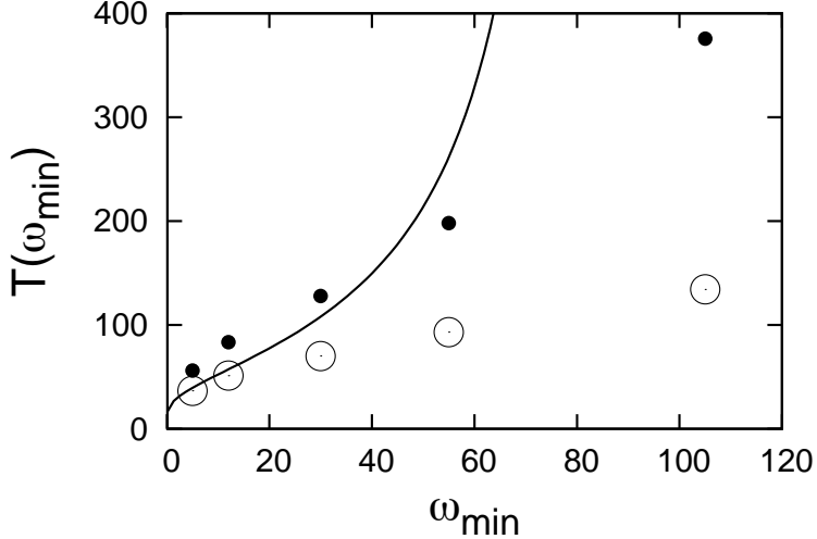
Figure 19: Temperature in different steady state keeping the forcing constant and varying the dissipation scale \omega_{\min} : big empty circles correspond to the temperature T_R on the right of the forcing scale, whereas small filled circles to the left side, T_L . The continuous line is the prediction (32).
