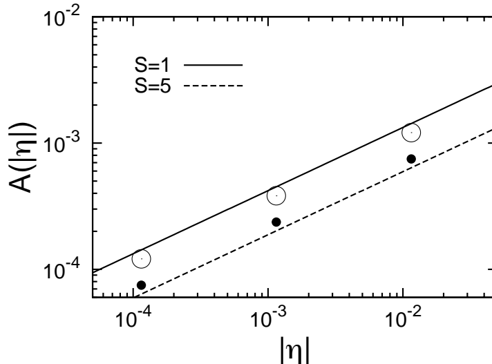
Figure 16: Results for the fitted values of the thermodynamic quantity A = e^{-\frac{h}{T}} plotted against the forcing levels, as obtained in the simulations shown in Fig. 4: the values of A_L are shown by filled circles while A_R by empty ones. The continuous and dashed lines refer to prediction (32) with S = 1 and S = 5 respectively.
