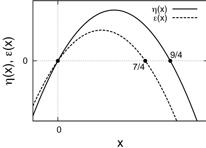
Figure 6: Energy and particle fluxes on power-law solutions n(\omega, t) \sim \omega^{-x} as functions of x for the three-dimensional hard sphere model.
