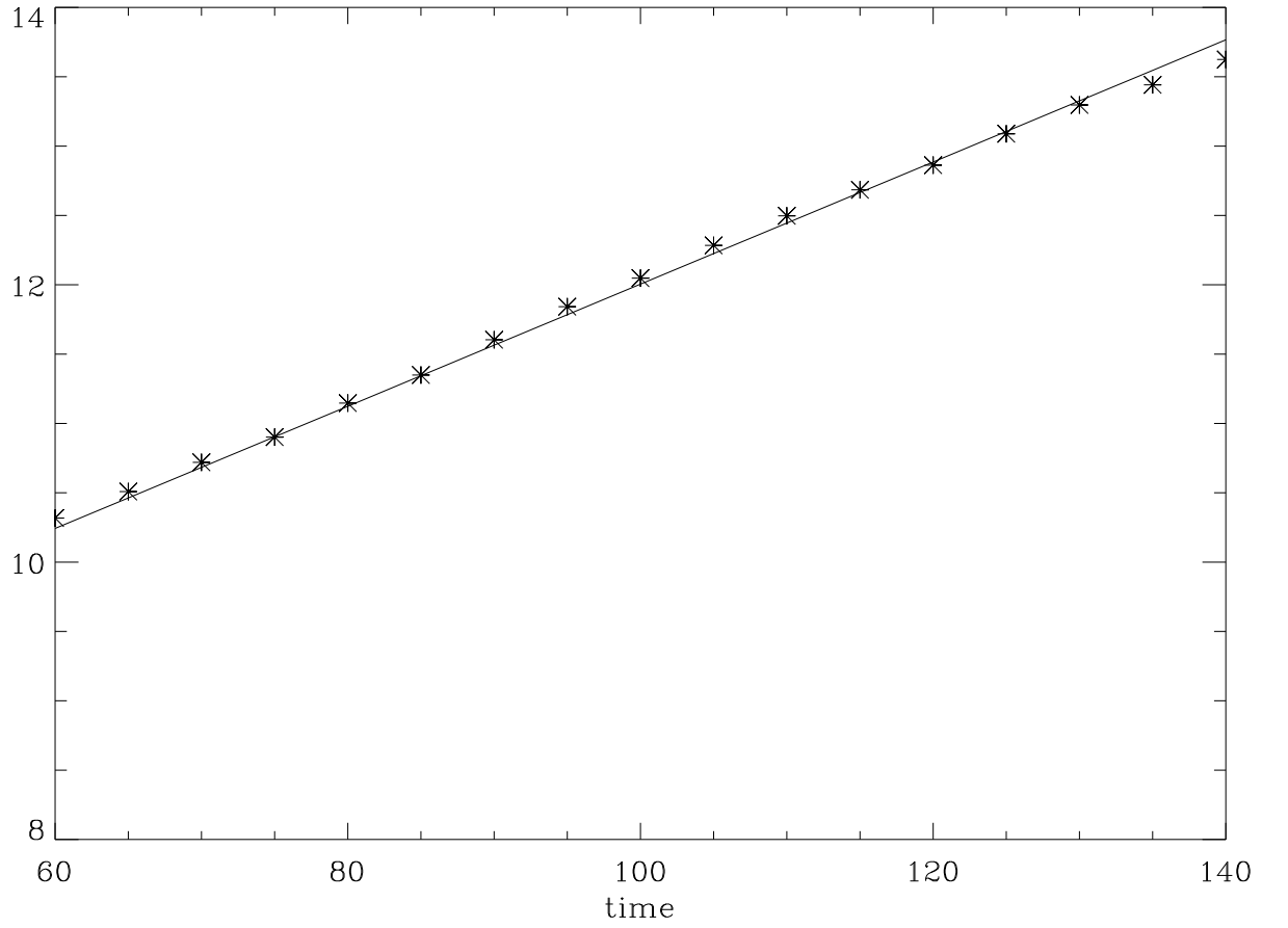
Figure 1. Growth in time of the fluid current density (continuous line) and of the kinetic current density (stars) at the X – point during the linear phase of the reconnection process.
