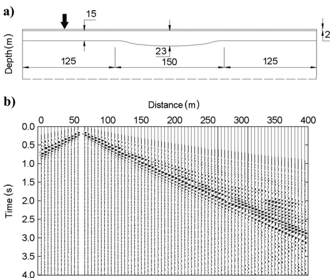
Figure 3. (a) Synthetic model geometry. (b) Synthetic seismogram for the shot position at 60 m—black arrow in (a).
