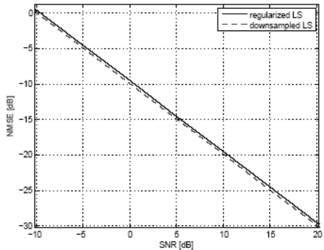
Fig. 5. Normalised MSE of the CIR estimate.
