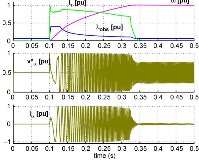
Fig. 8. Simulation-Speed step 0 \div 10\,000 r/min at no-load. Scale factors: \omega : 10\,000 r/min/p.u., \hat{\lambda} : 1 V · s/p.u., i_\tau : 45 A/p.u., v_\alpha^* : 230 V/p.u., i_\alpha : 45 A/p.u.
