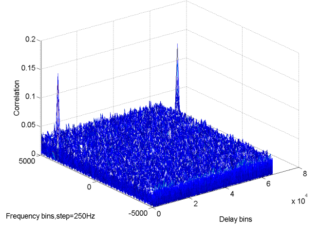
Figure 5: CAF envelope of the Galileo OS signal evaluated by the two steps method for a C/N_0 of 45 dBHz with bit transition.
