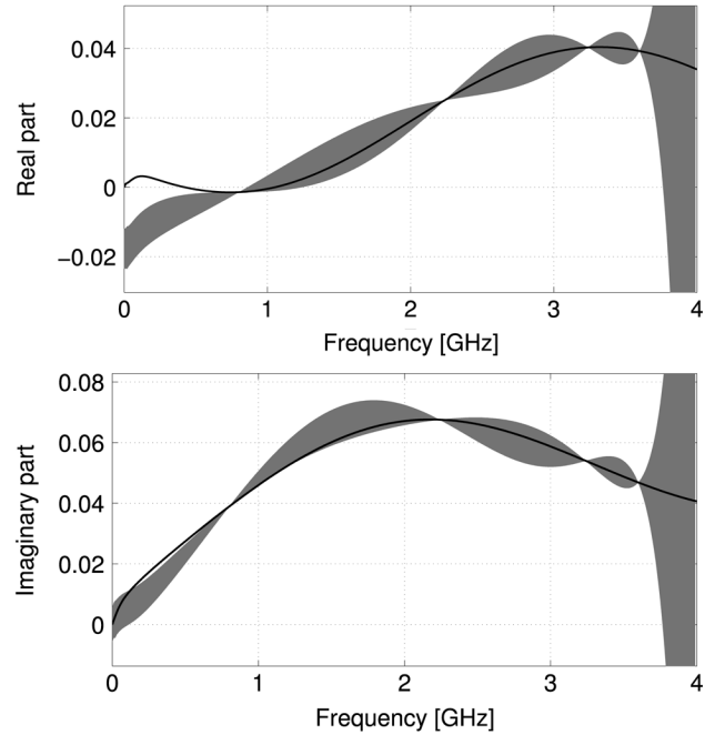
Fig. 9. Check for causality of S_{11} , based on computation of generalized Hilbert transform. Since continuous line (representing raw data) is outside gray area (computed Hilbert transform inclusive of a frequency-dependent error bar), dataset is noncausal.
