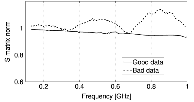
Fig. 13. Norm of S matrix: values greater than one denote passivity violations.
