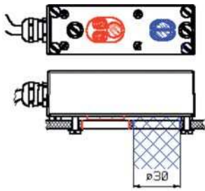
Fig. 5 - Sensore ad infrarossi con componenti passive, in blu, ed attive, in rosso. Infra-red sensor with passive components in blue and active components in red.
