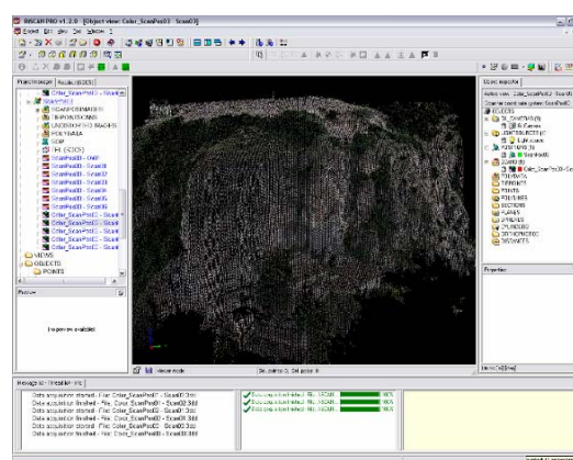
Figure 7. Acquisition Software - RiscanPro - Riegl – scan position 03.
