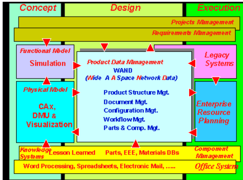
Figure 2: WAND architecture
