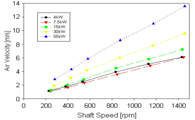
Fig. 5. Fin channel inlet air velocity versus the rotor speed for the TEFC induction motors shown in Fig. 3.
