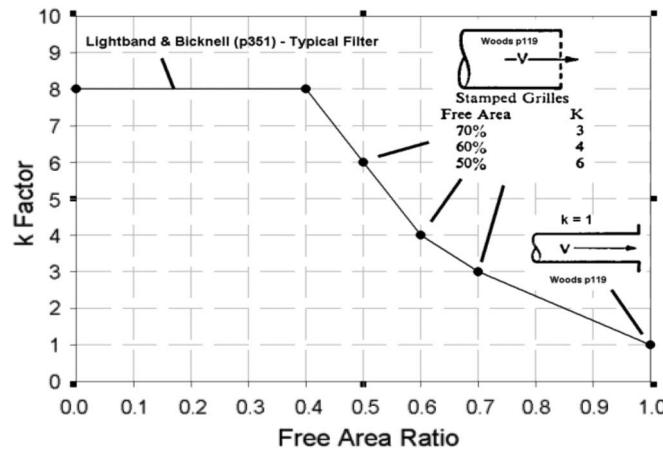
Fig. 13. Outlet grill k factor.
