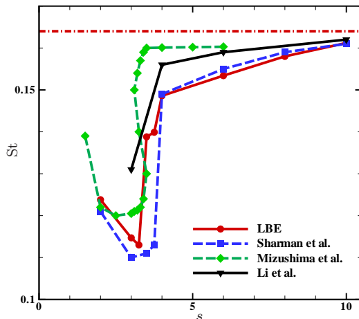
Fig. 11. Flow past two tandem cylinders at Re = 100 . The dependence of the Strouhal number St on the dimensionless spacing s between two cylinders. The LBE results are compared with that of Li et al. [33], Sharman et al. [38] and Mizushima & Suehiro [37]. The dash-dot line indicates the value of St \approx 0.164 for a single cylinder in an unbounded domain at Re = 100 .
