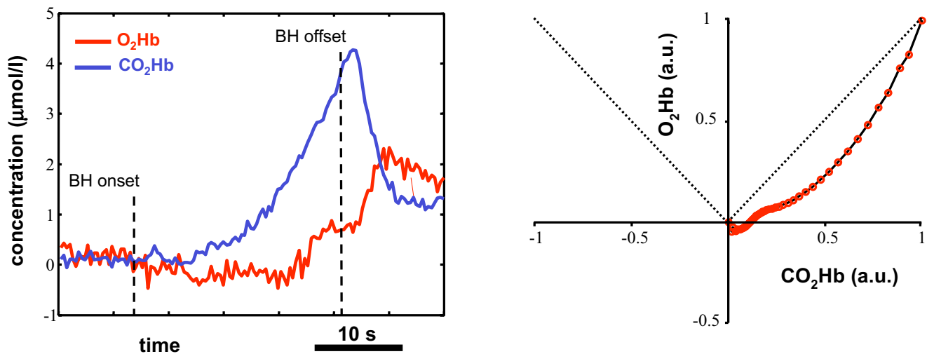
Figure 9 NIRS signals and VMR pattern for subject A. Time course of the \text{O}_2\text{Hb} and \text{CO}_2\text{Hb} concentration signals for subject A (healthy current smoker) during BH (left panel) and bidimensional VMR pattern (right panel). The signals reveal an uncompensated increase of the \text{CO}_2\text{Hb} level, that determines a VMR pattern always out of the two bisectors region. Also, the onset of VMR is delayed and the VMR pattern never reaches a plateau condition.
