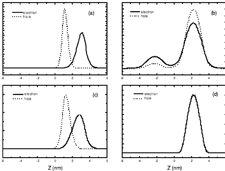
FIG. 8. Electron and hole particle distribution along the growth direction for two coupled dots of, respectively, 2.5 nm and 2.7 nm of height, separated by a 2.5 nm AlN barrier. The dot parameter sets corresponds to: (a) GaN, except valence/conduction band offset (GaAs one); (b) GaAs; (c) GaN, except electron/hole masses (GaAs ones); (d) GaN, except that the electric field is set to zero.
