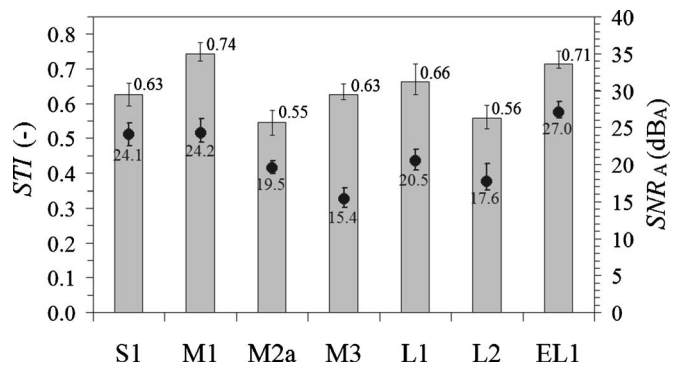
FIG. 2. Mean STI (gray blocks) and SNR_A (black circles) values and min-max range bars for seven of the eight classroom types.
