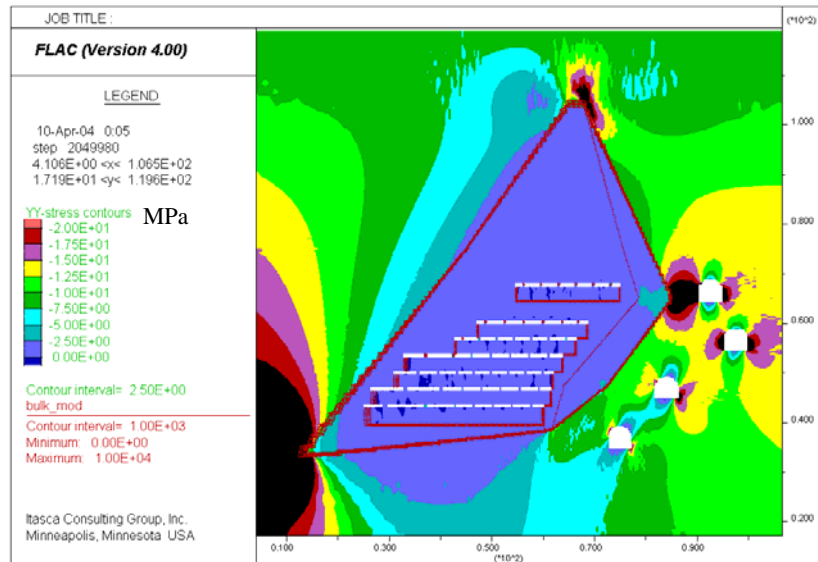
Figure 8. Vertical stresses in the orebody at the end of exploitation (the values larger than 20MPa are in black)
