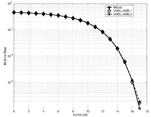
Fig. 1. BER curves: Matlab vs. VHDL-AMS 1 and VHDL-AMS 2.
