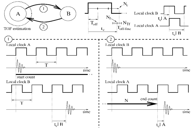
Fig. 3. Two-Way-Ranging scheme.
