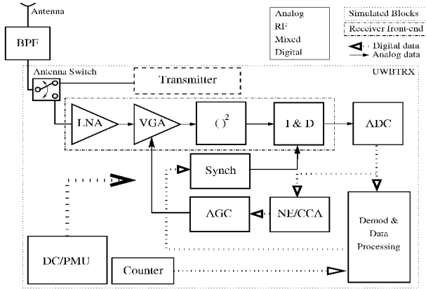
Fig. 2. Receiver structure.
