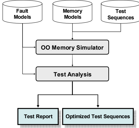
Figure 1. Simulator architecture
