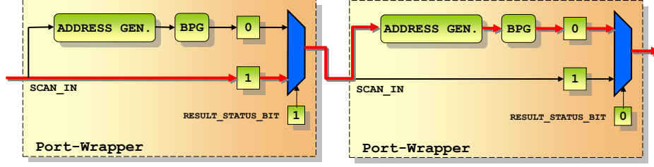
Figure 4: Results_Scan_Chain
