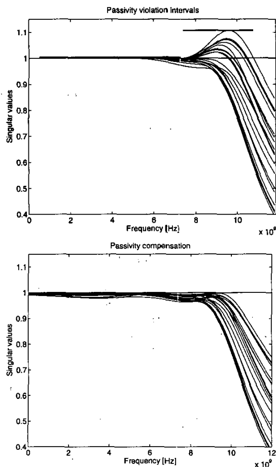
Figure 5: Passivity compensation for a macromodel of a multiple via structure. The singular values are plotted versus frequency for the non-passive macromodel (top panel) and for the passive macromodel (bottom panel).
