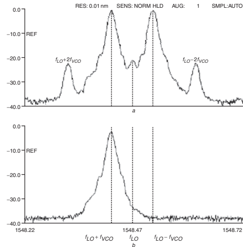
Fig. 2 OVCO output and RX signal optical spectra when two signals phase-locked
