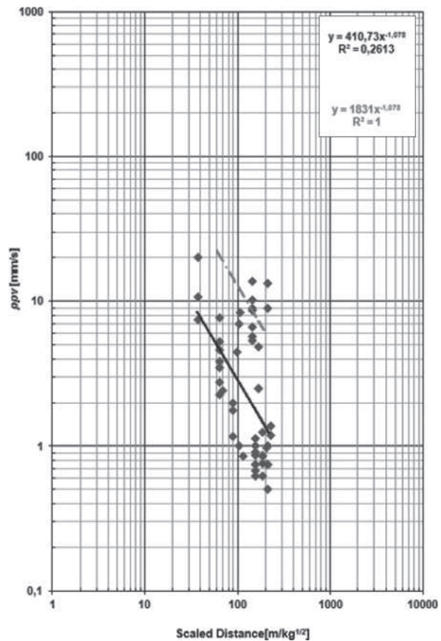
Fig. 11. Site law pertaining to the blast records when the “Along the strike” bench orientation was employed. The regression analysis provides a very low correlation. The dashed line represents the transposition of the curve that provides a confidence level of 95%.
