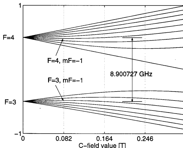
Fig. 1. Breit-Rabi law for Cs atoms.
