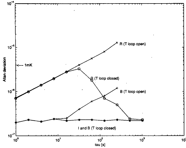
Fig. 6. Stability of the excitation current I (with the current loop closed) of the average magnetic field B (both in open and closed temperature loop) and of the coil resistance R (also in both open and closed temperature loop).
