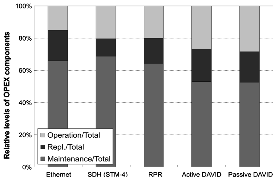
Fig. 11. Relative levels of OPEX components, averaged over the 20-, 40-, and 80-G cases.
