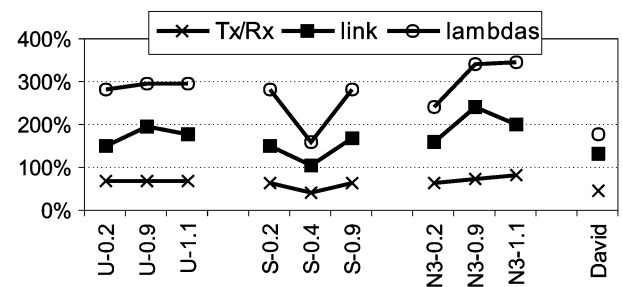
Fig. 13. Cost ratio passive/active; x -axis labels denote demand ( U = \text{Uni} , S = \text{Serv} , and N3 = \text{Neigh3} ; the number after the dash is the value of d ).
