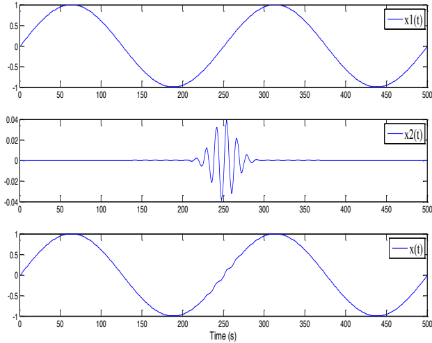
Figure 1. The simulated signal and its high and low frequency components
